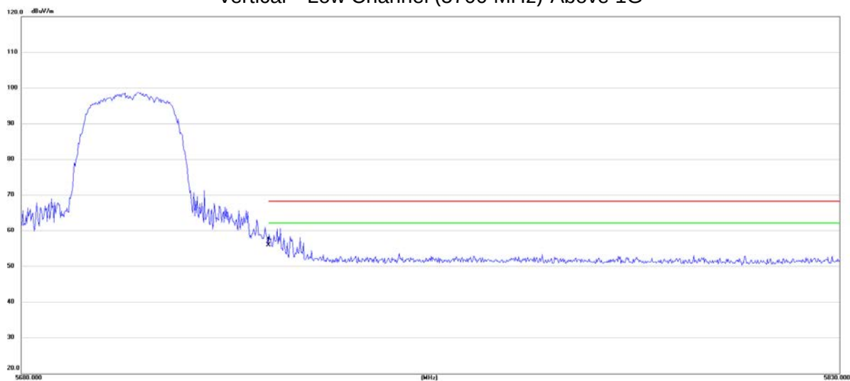
Vertical Low Channel (5700 MHz)-Above 1G
