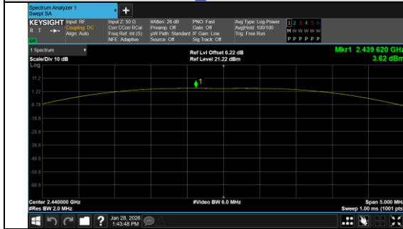
Peak Output Power BLE 2M_Channel 19
