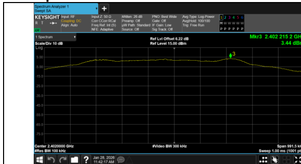
In-Band Reference Level BLE 1M_Channel 0
