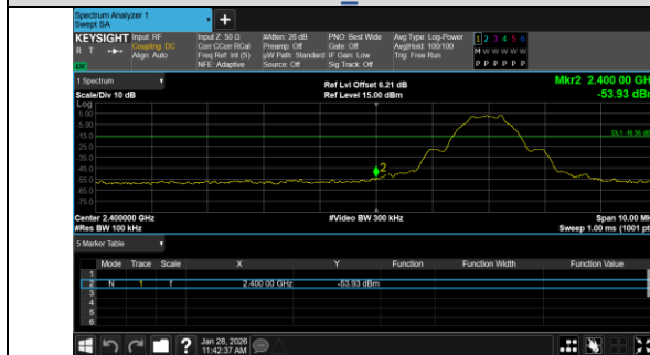
Out Of Band Emission BLE 1M_Channel 0
