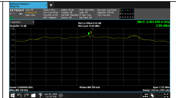
In-Band Reference Level BLE 2M_Channel 1
