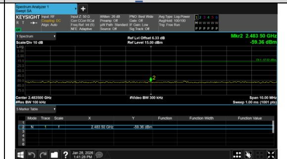
Out Of Band Emission BLE 2M_Channel 1
