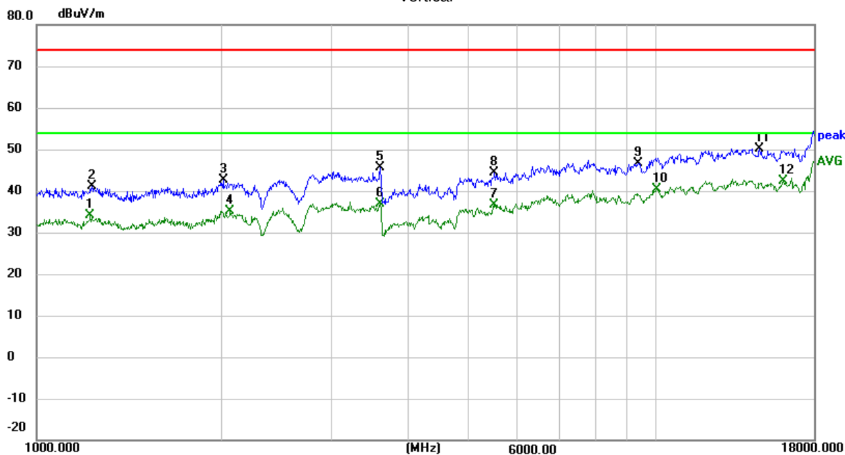
High Channel (2480 MHz)(GFSK)-- Above 1G Vertical
