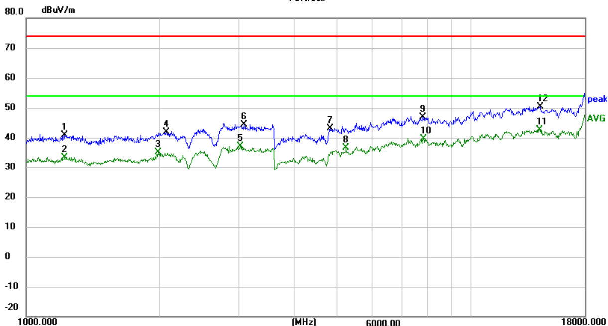
Low Channel (2402 MHz)(GFSK)--Above 1G Vertical
