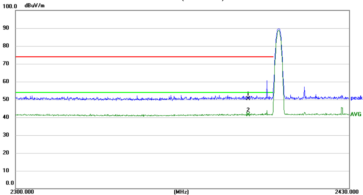
Vertical Low Channel (2402 MHz)-Above 1G
