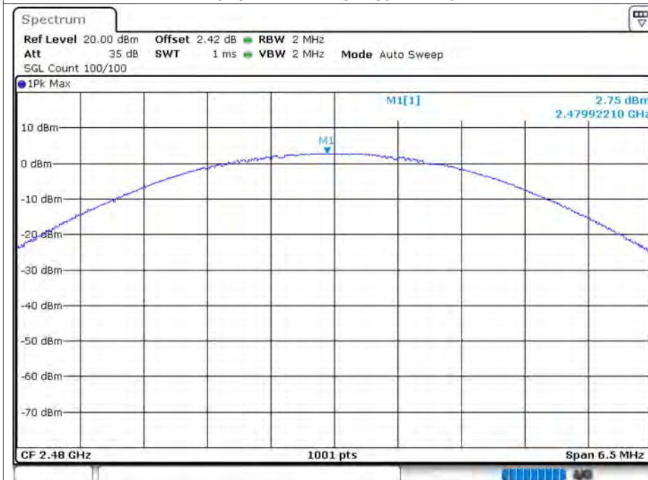
Power NVNT 2-DH5 2480MHz Ant1
