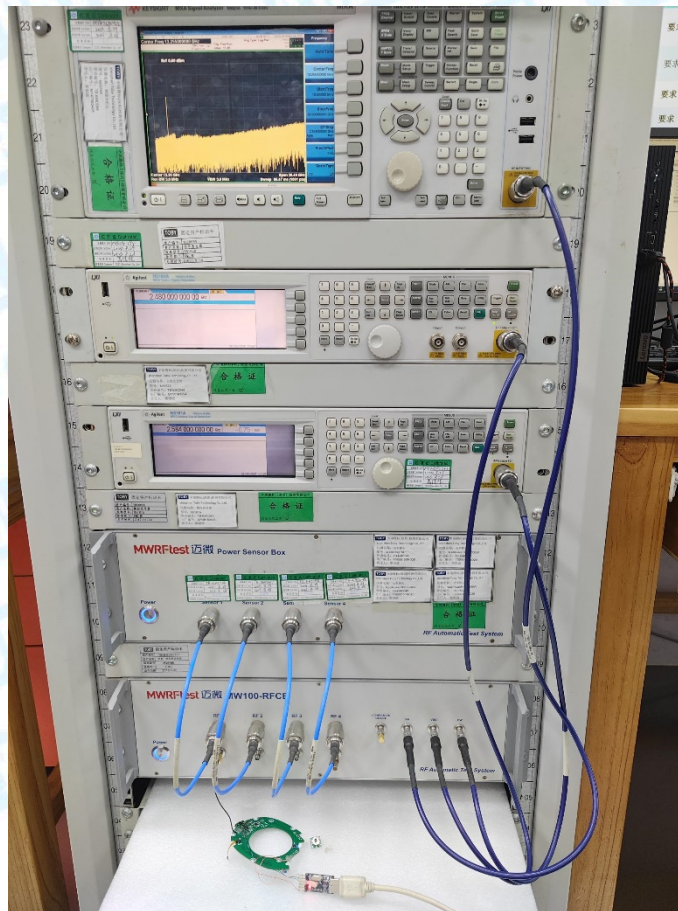
Photo of Setup for Conducted Measurement
