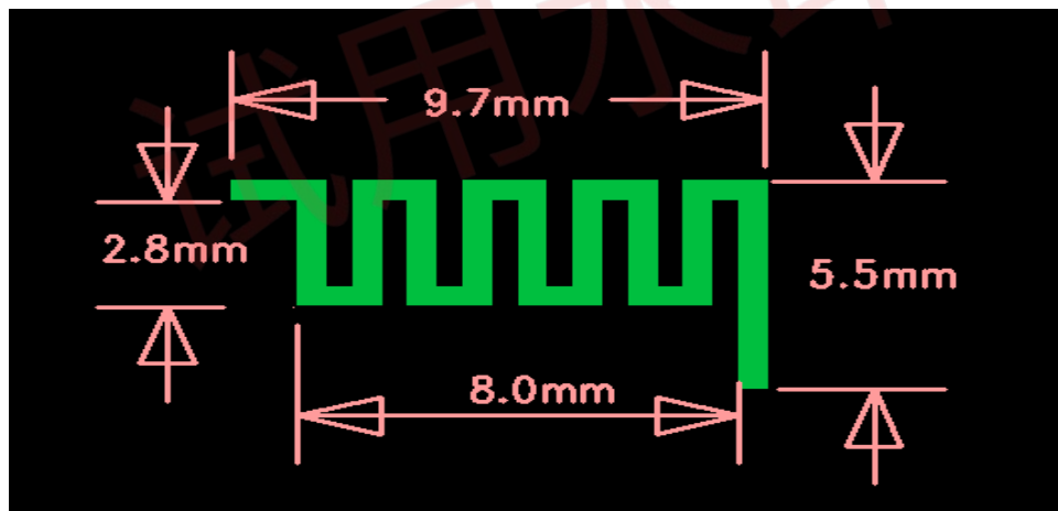
Antenna Photo & Length (mm)
