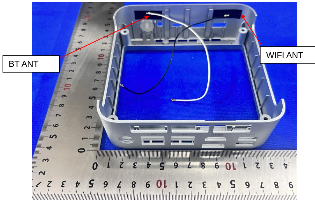
Internal photos
