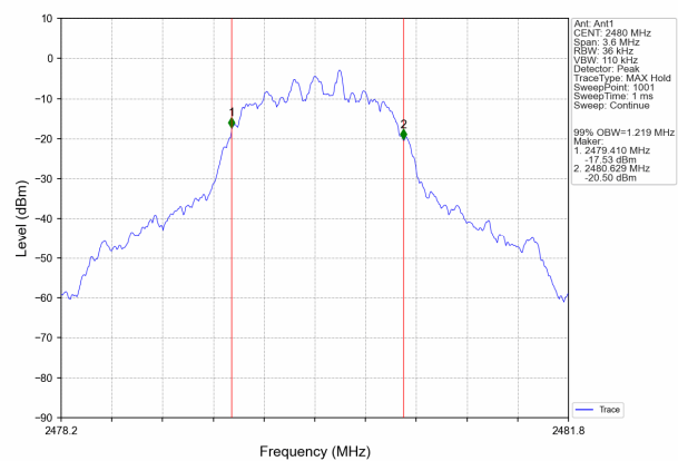
\pi/4 DQPSK High Channel
