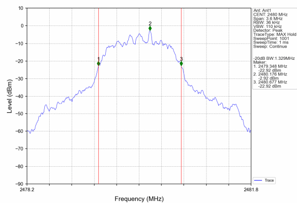
\pi/4 DQPSK High Channel
