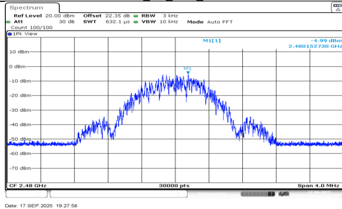
BLE_1M_Ant1_2480
