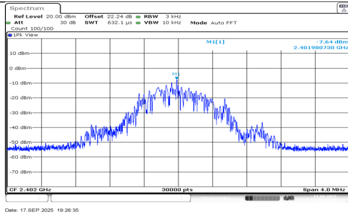
BLE_1M_Ant1_2402
