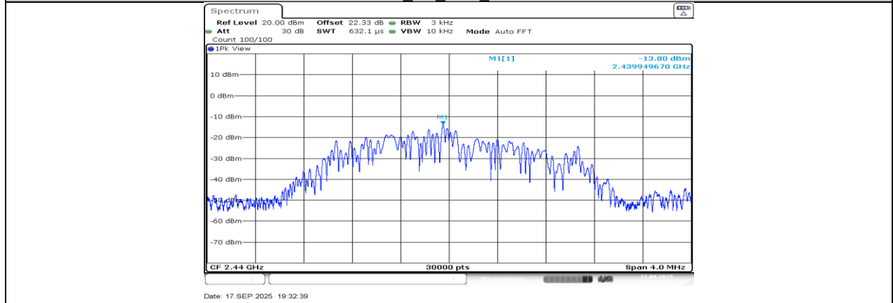
BLE_2M_Ant1_2440
