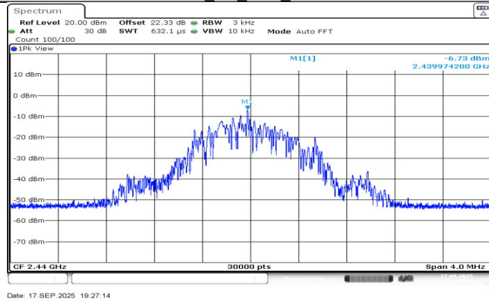
BLE_1M_Ant1_2440
