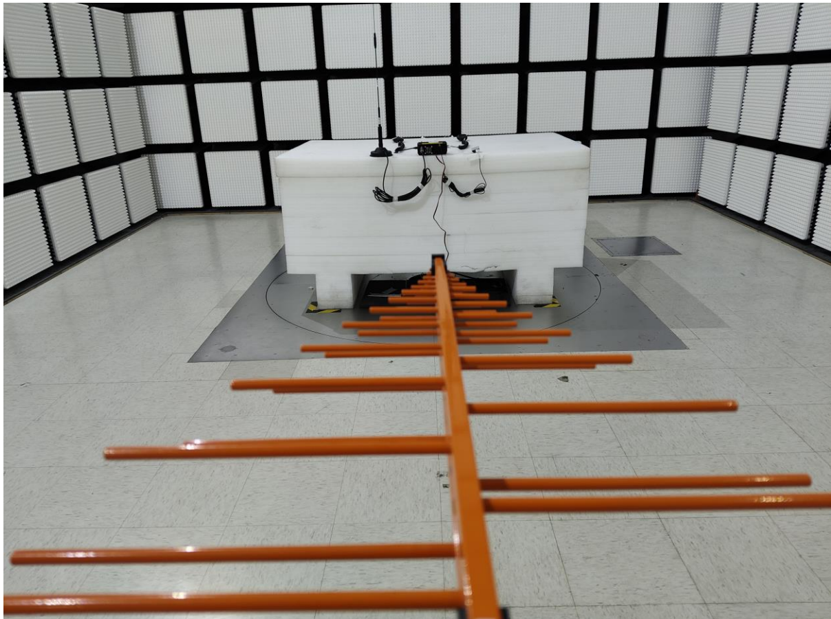
Radiated Emission 30 MHz-1 GHz Rear View M1
