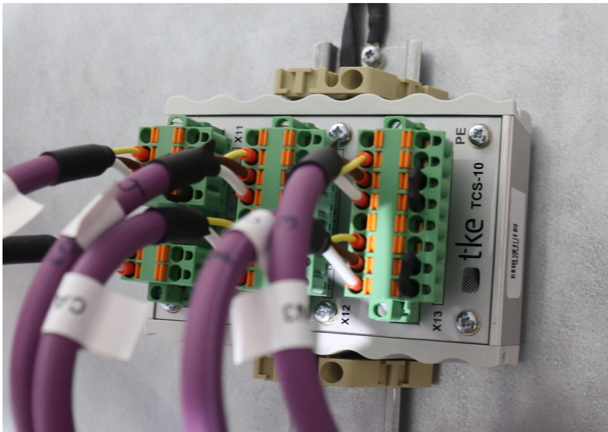
Photograph 1. The EUT
