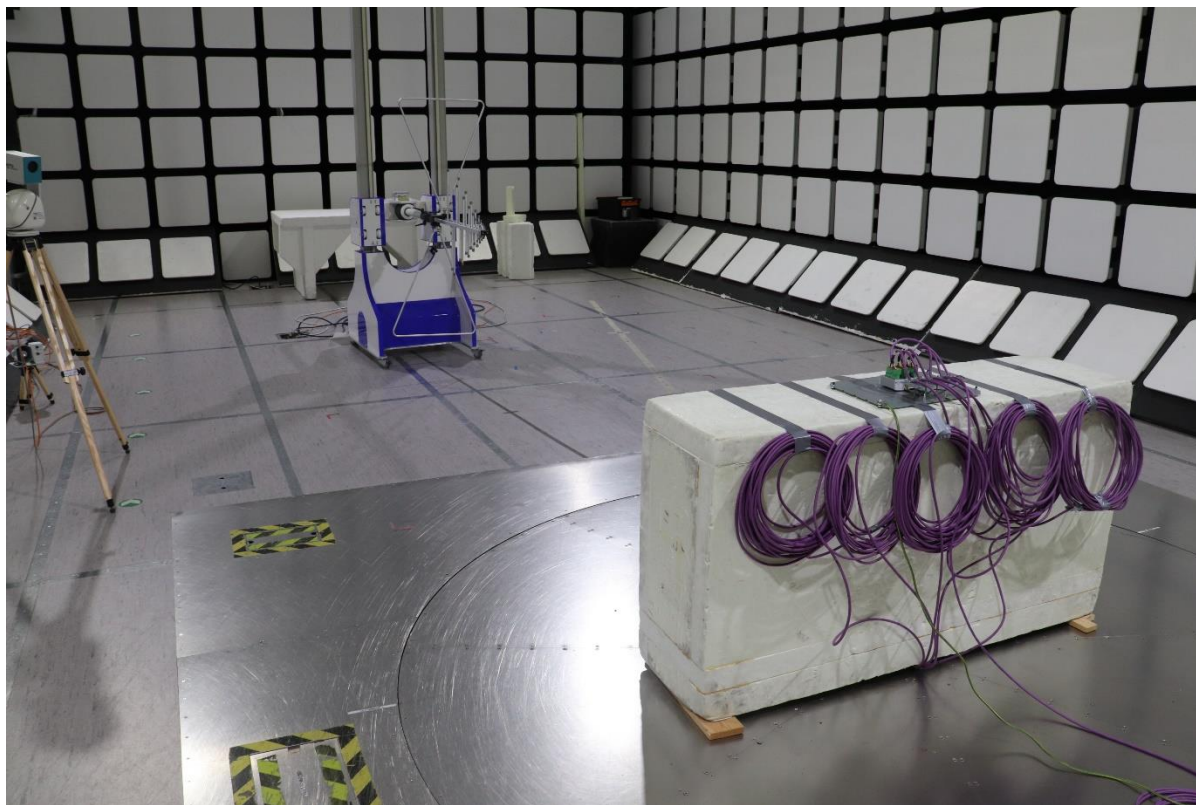
Photograph 2. Radiated Emissions 30 – 1000 MHz
