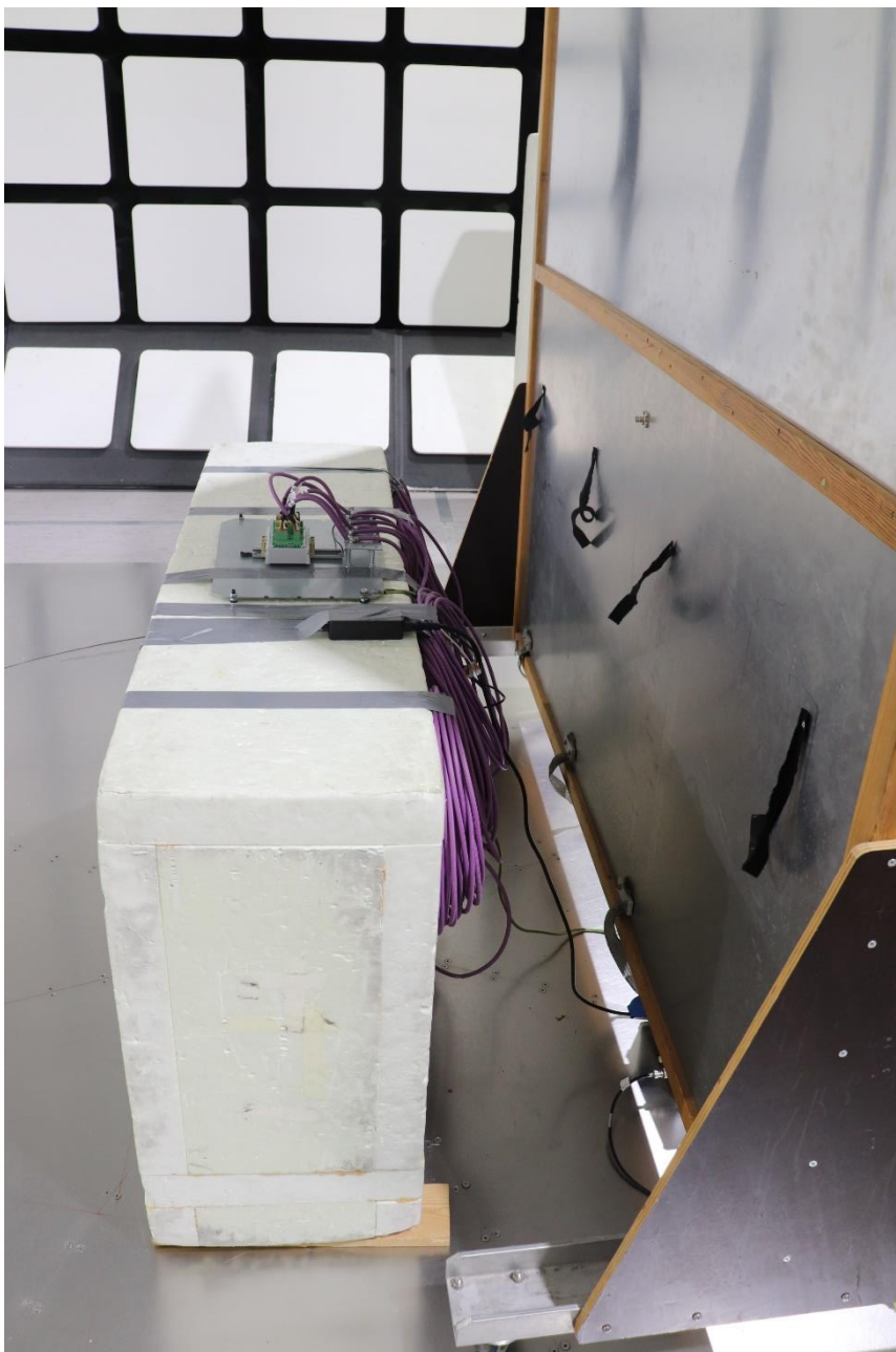
Photograph 3. Conducted Emissions
