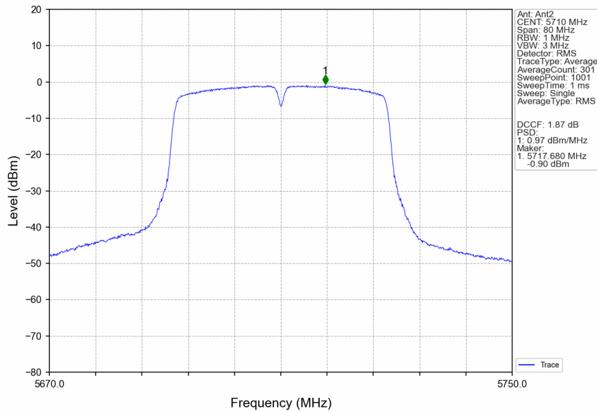
802.11ac(VHT40)_HCH_5710MHz_MIMO_NTNV
