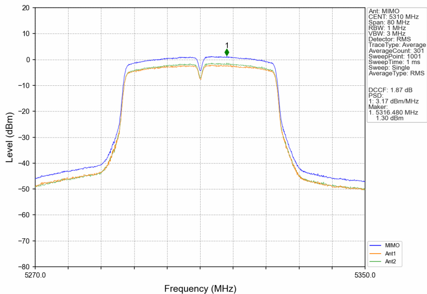
802.11ac(VHT40)_HCH_5310MHz_MIMO_NTNV
