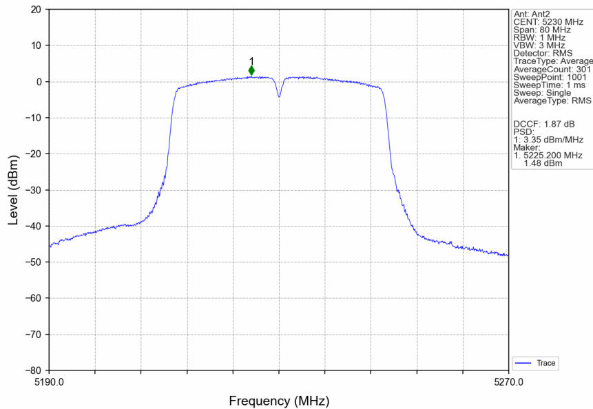
802.11ac(VHT40)_HCH_5230MHz_MIMO_NTNV
