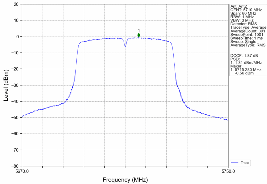
802.11n(HT40)_HCH_5710MHz_MIMO_NTNV
