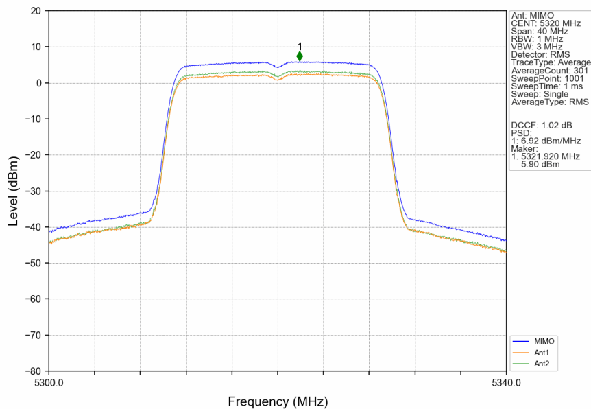
802.11ac(VHT20)_HCH_5320MHz_MIMO_NTNV
