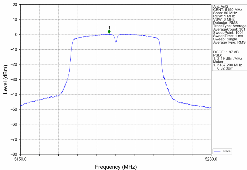
802.11ac(VHT40)_LCH_5190MHz_Ant2_NTNV
