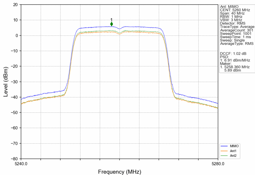
802.11ac(VHT20)_LCH_5260MHz_MIMO_NTNV
