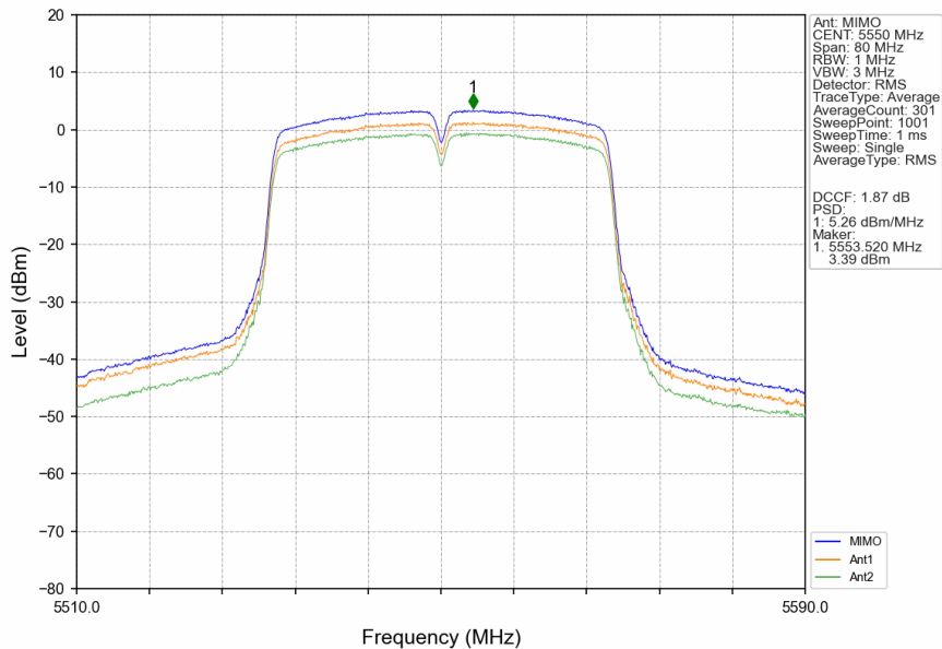
802.11ac(VHT40)_MCH_5550MHz_MIMO_NTNV
