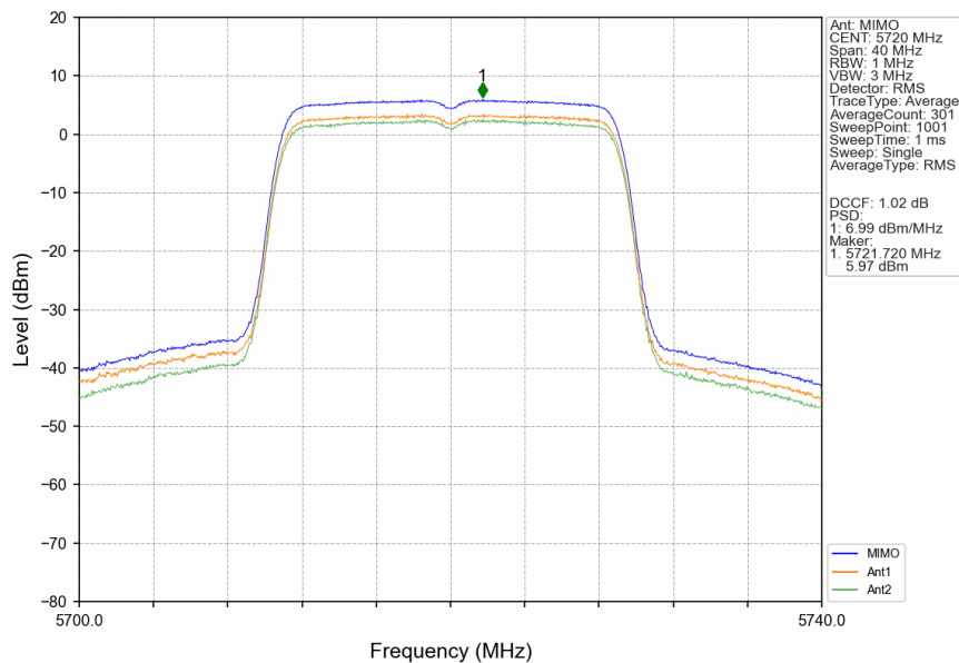
802.11ac(VHT20)_HCH_5720MHz_MIMO_NTNV
