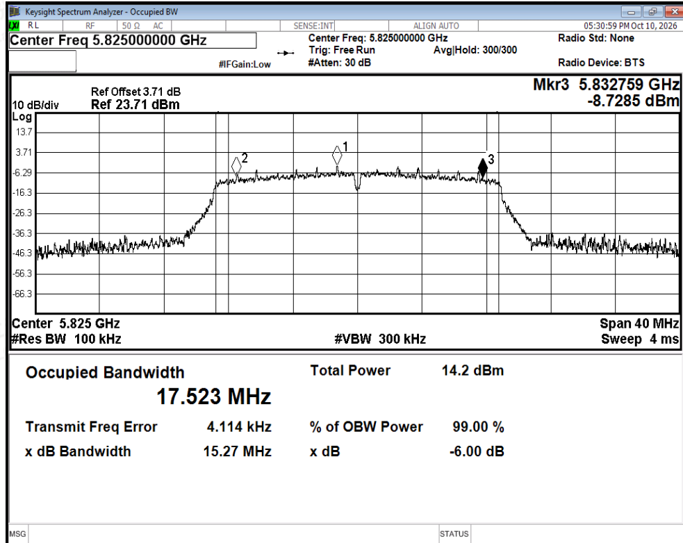
-6dB Bandwidth NVNT ac20 5825MHz Ant1
