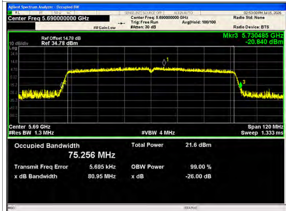
-26dB Bandwidth NVNT ac80 5690MHz Ant1
