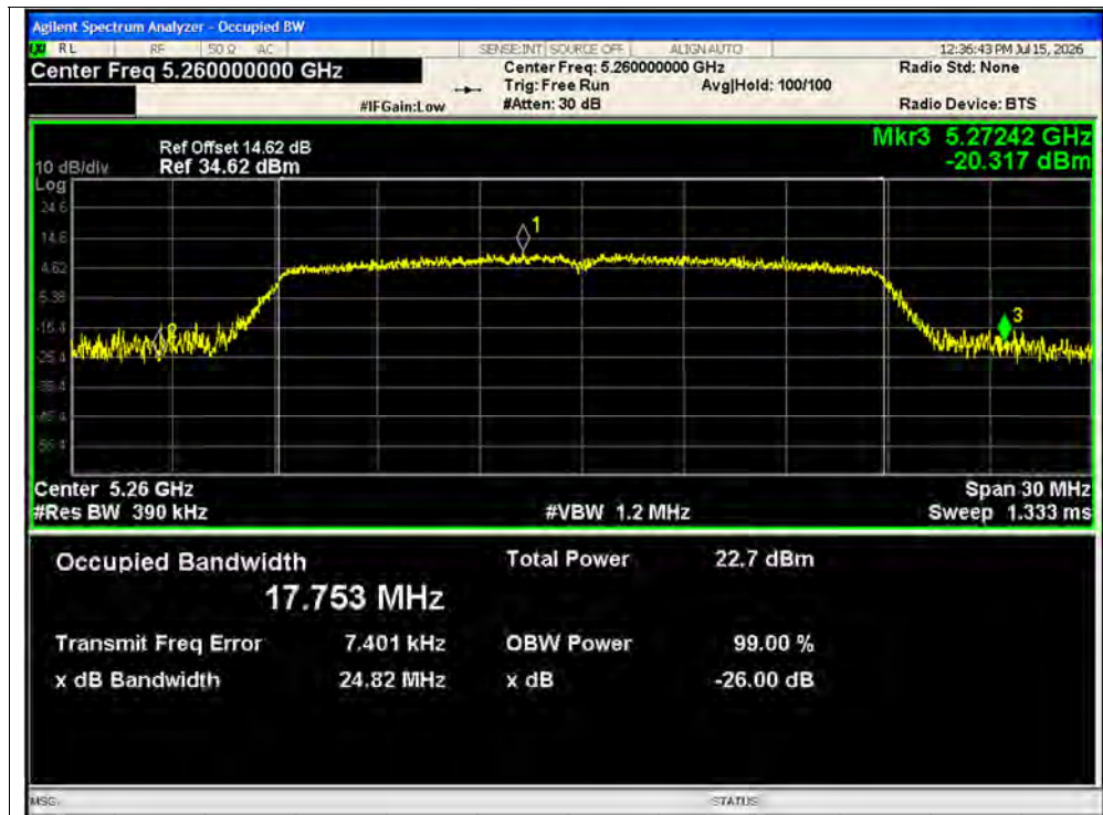
-26dB Bandwidth NVNT ac20 5260MHz Ant1
