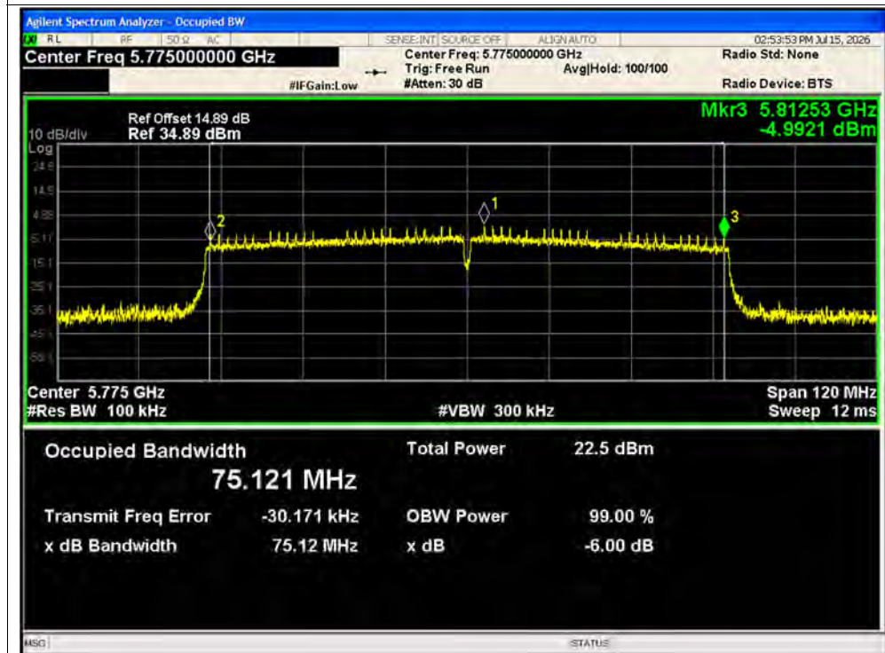
-6dB Bandwidth NVNT ac80 5775MHz Ant1
