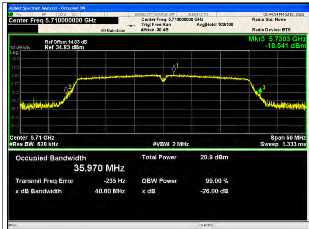
-26dB Bandwidth NVNT ac40 5710MHz Ant1
