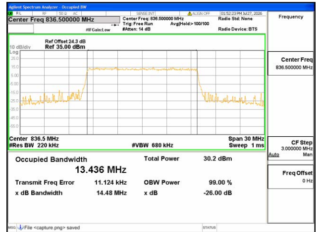
B26 Part22 / 15MHz / QPSK/ Mid CH
