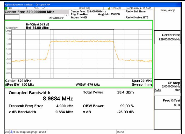
B26 Part22 / 10MHz / 64QAM/ Low CH
