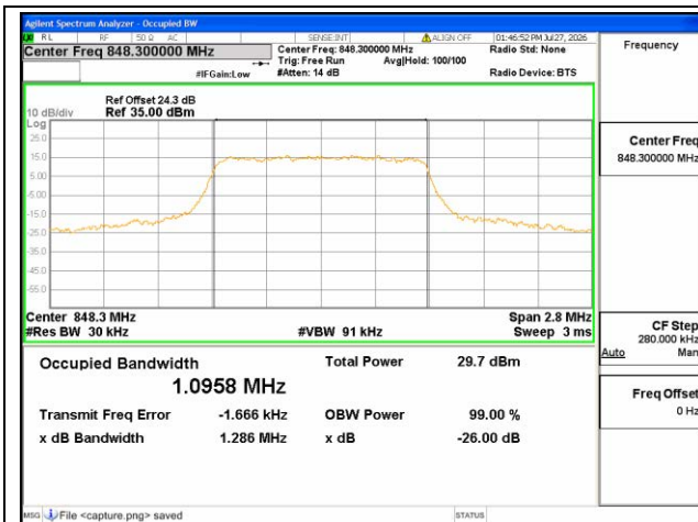
B26 Part22 / 1.4MHz / QPSK/ High CH
