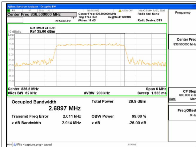
B26 Part22 / 3MHz / QPSK/ Mid CH
