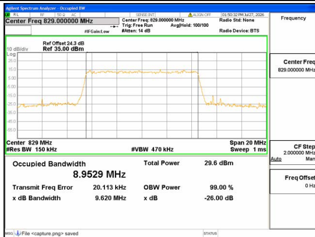
B26 Part22 / 10MHz / 16QAM/ Low CH
