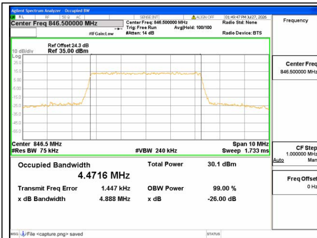
B26 Part22 / 5MHz / QPSK/ High CH
