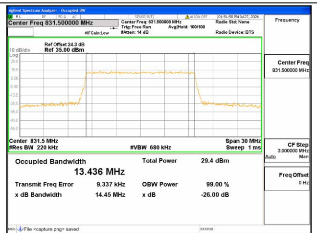
B26 Part22 / 15MHz / 16QAM/ Low CH
