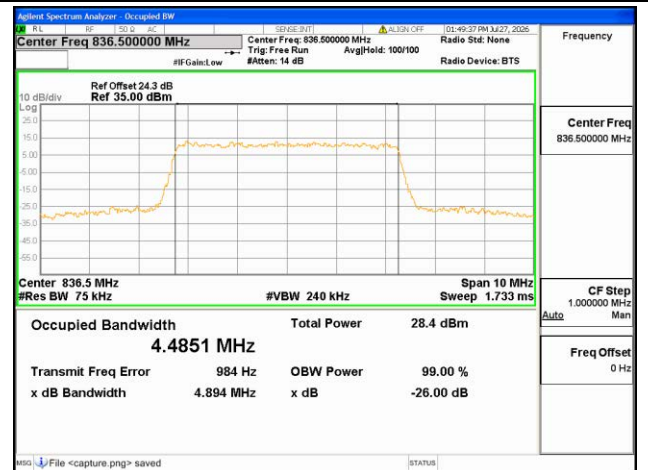
B26 Part22 / 5MHz / 64QAM/ Mid CH
