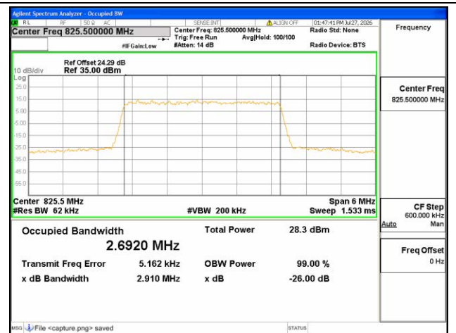
B26 Part22 / 3MHz / 64QAM/ Low CH
