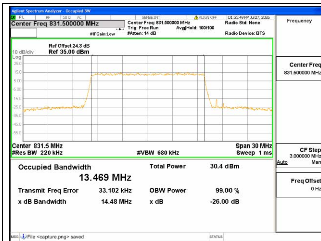
B26 Part22 / 15MHz / QPSK/ Low CH
