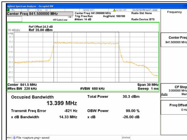
B26 Part22 / 15MHz / QPSK/ High CH
