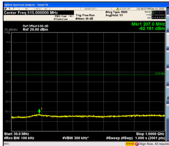
Band66_1.4MHz_QPSK_132322_6RB#0_30~1000_30~1000
