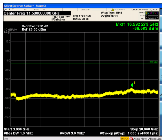
Band66_1.4MHz_QPSK_132322_6RB#0_3000~20000_3000~20000
