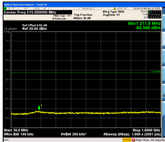
Band66_1.4MHz_QPSK_132322_6RB#0_30~1000_00_30~1000
