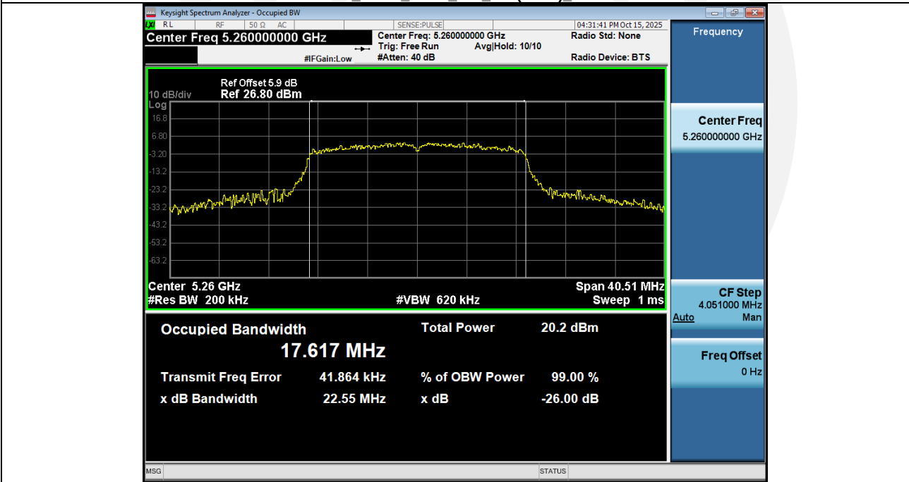
-26BW_NVNT_ANT1_802_11n(HT20)_5260
