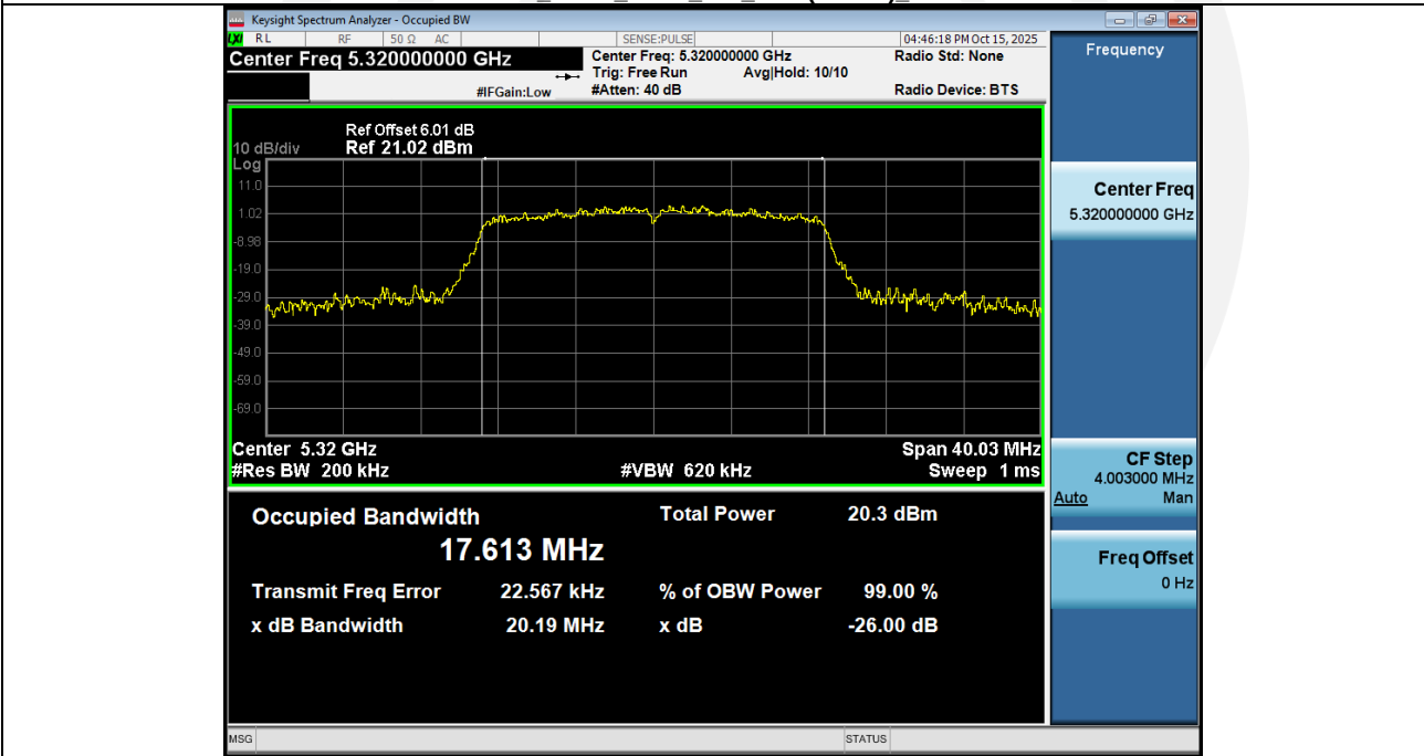
-26BW_NVNT_ANT1_802_11ac(VHT20)_5320
