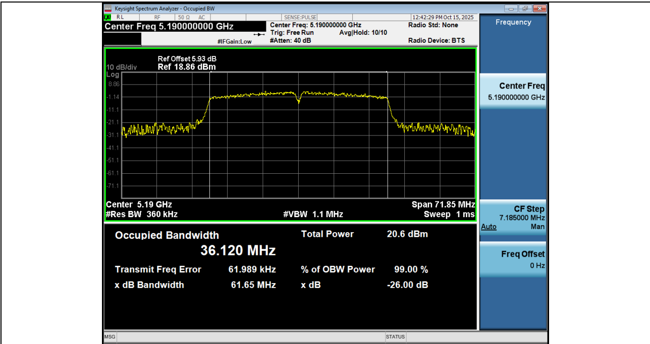
-26BW_NVNT_ANT1_802_11n(HT40)_5190
