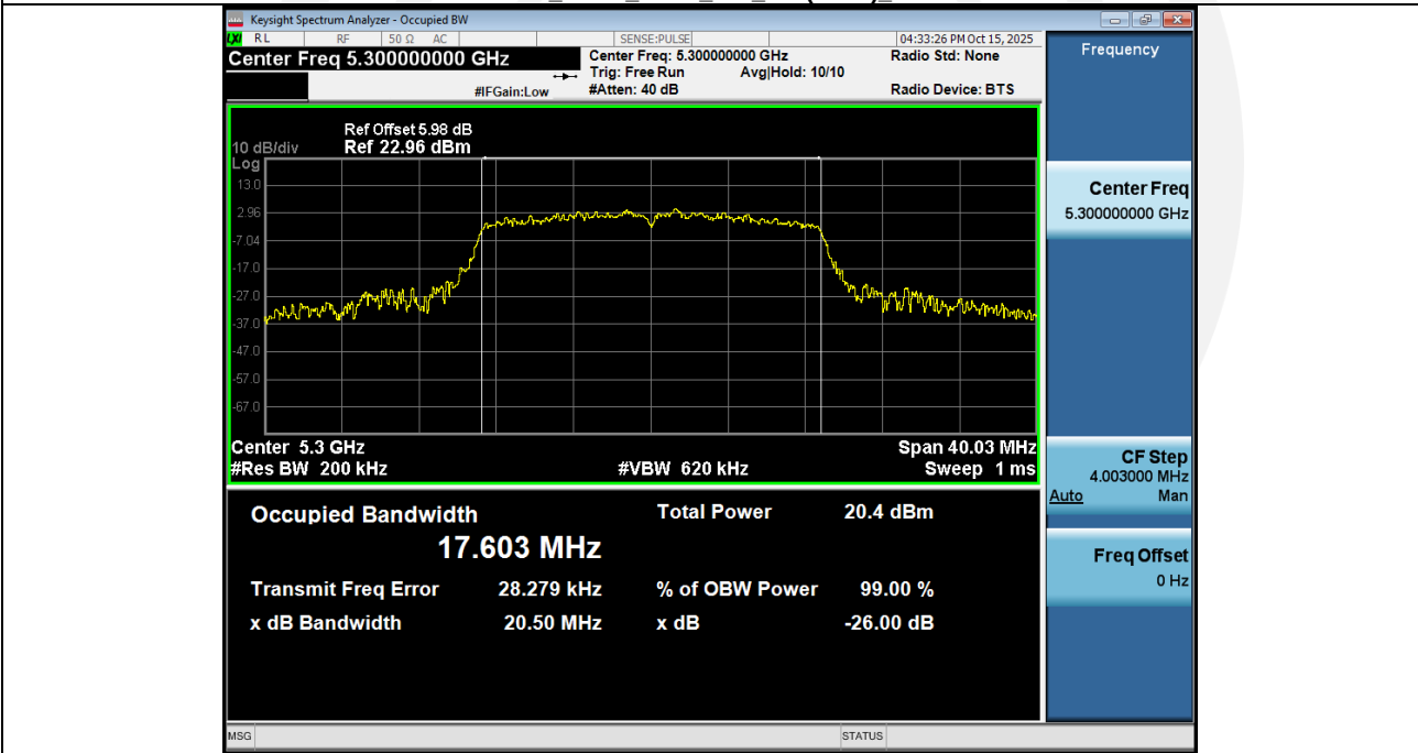
-26BW_NVNT_ANT1_802_11n(HT20)_5300
