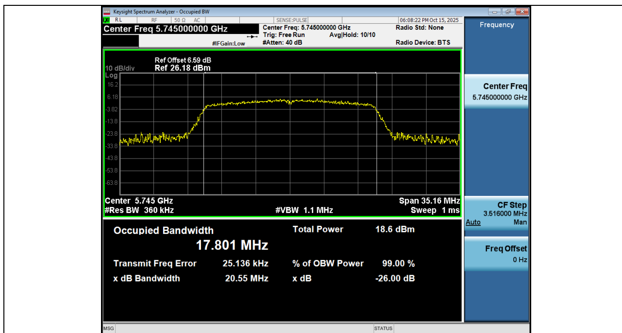
-26BW NVNT ANT1 802 11ac(VHT20) 5745
