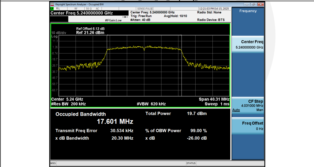
-26BW_NVNT_ANT1_802_11n(HT20)_5240
