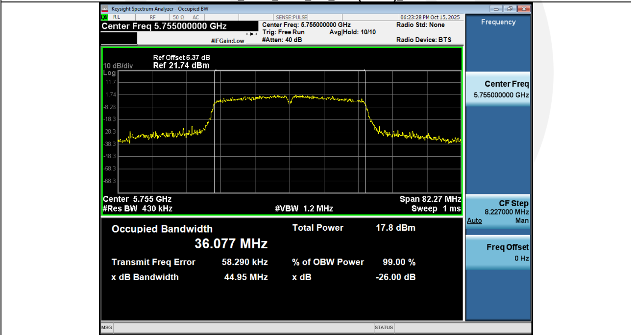
-26BW_NVNT_ANT1_802_11ac(VHT40)_5755
