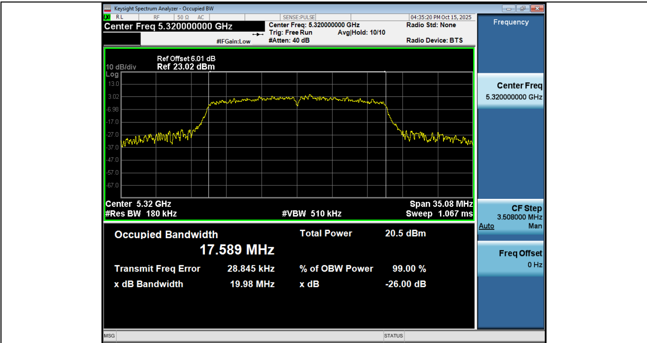
-26BW_NVNT_ANT1_802_11n(HT20)_5320
