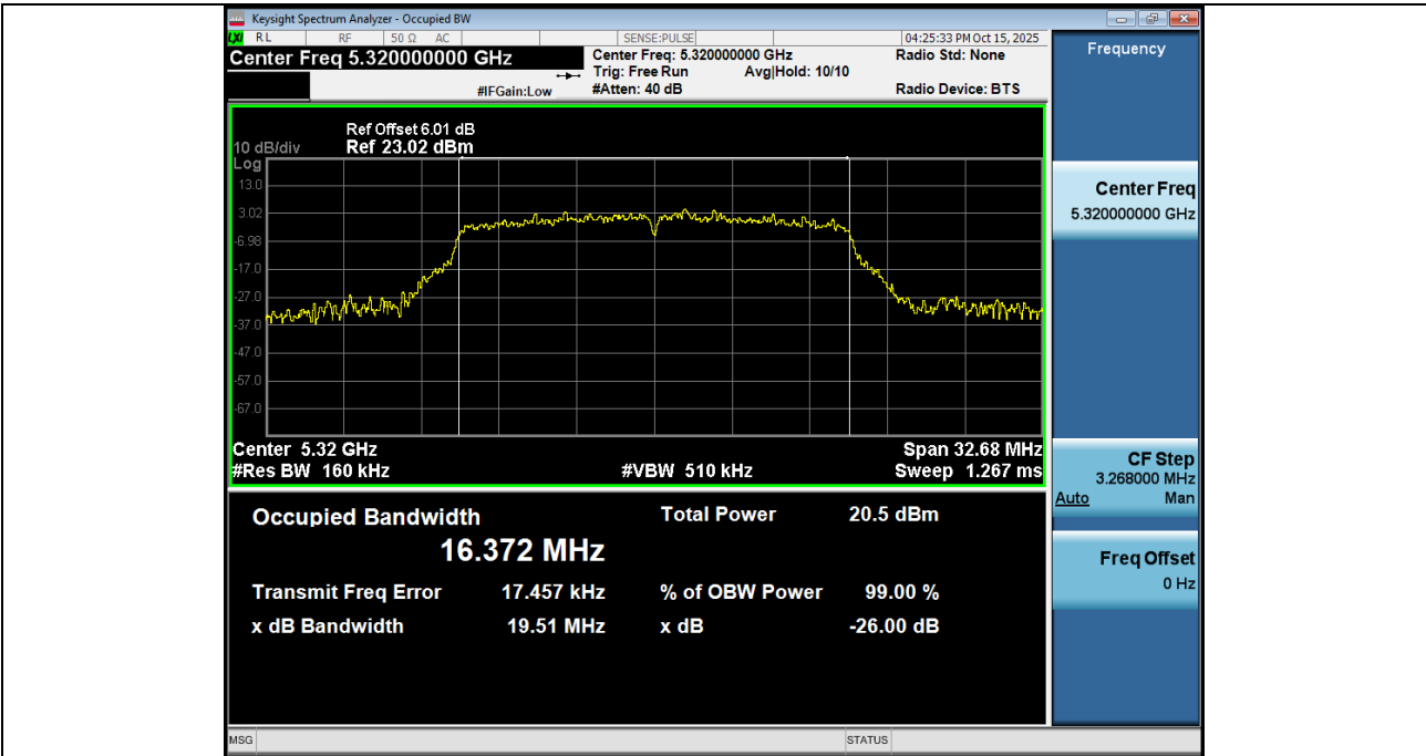
-26BW_NVNT_ANT1_802_11a_5320
