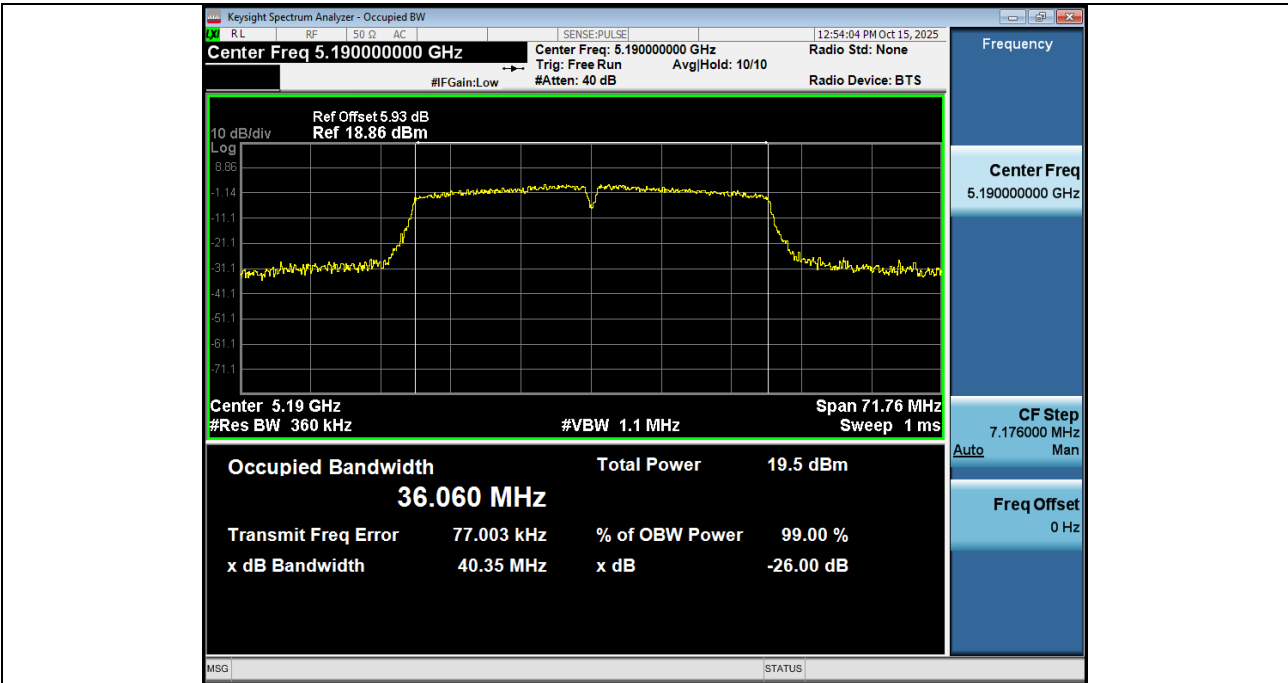
-26BW_NVNT_ANT1_802_11ac(VHT40)_5190
