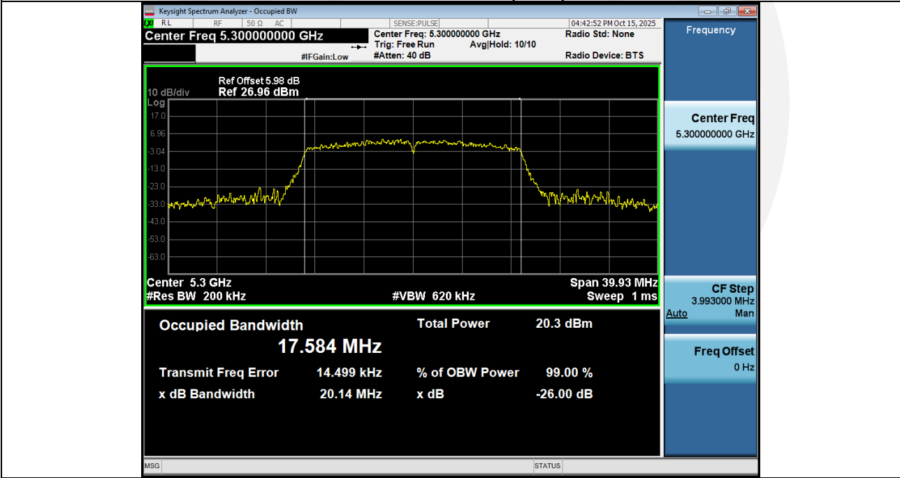
-26BW_NVNT_ANT1_802_11ac(VHT20)_5300
