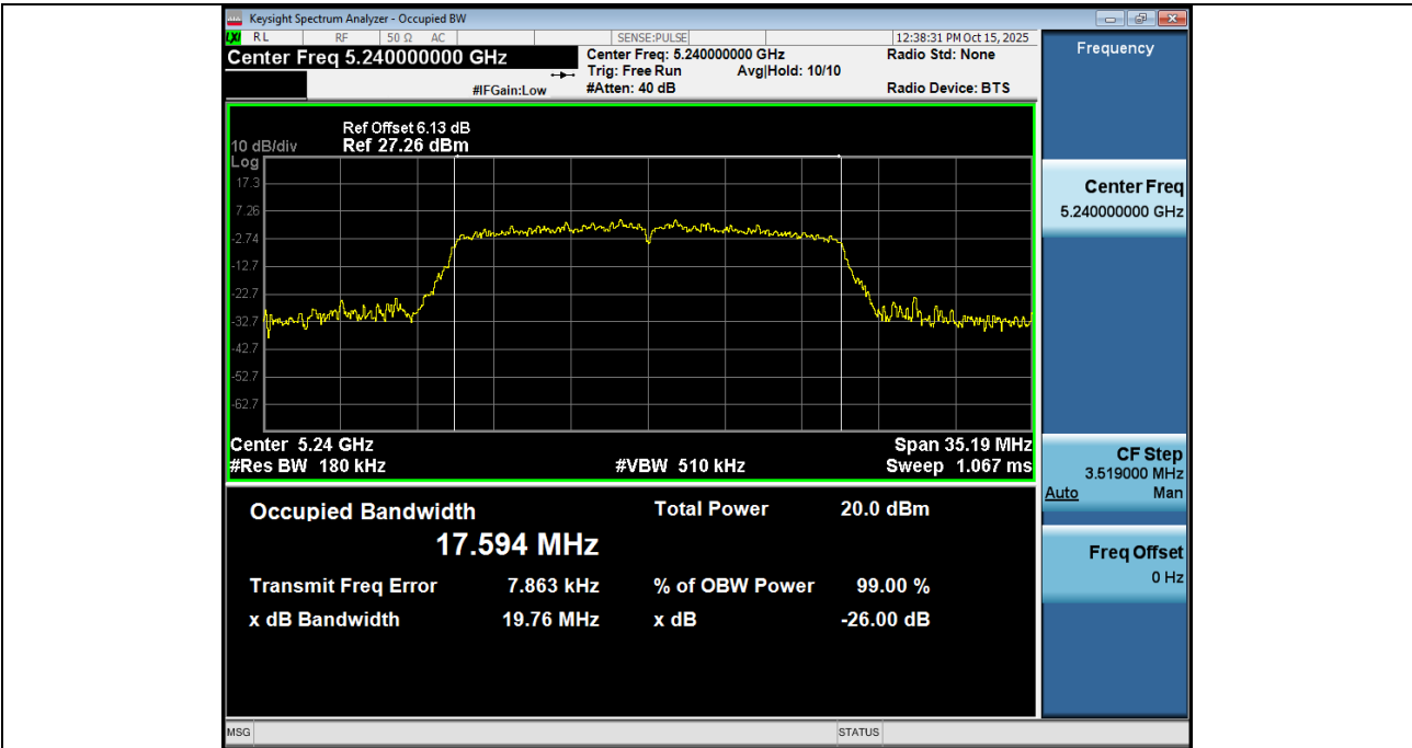
-26BW_NVNT_ANT1_802_11ac(VHT20)_5240
