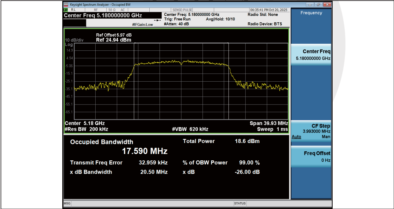
-26BW_NVNT_ANT1_802_11n(HT20)_5180
