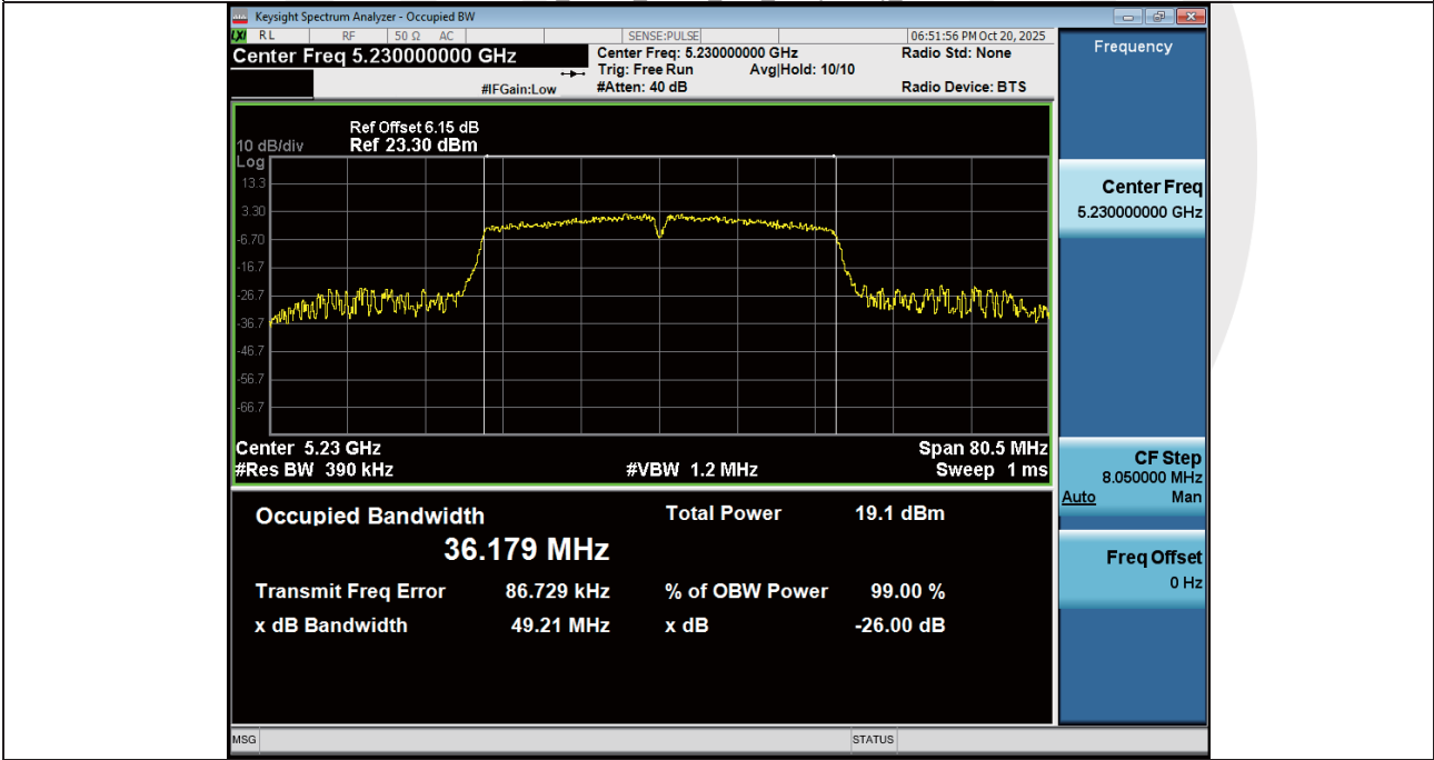
-26BW_NVNT_ANT1_802_11n(HT40)_5230
