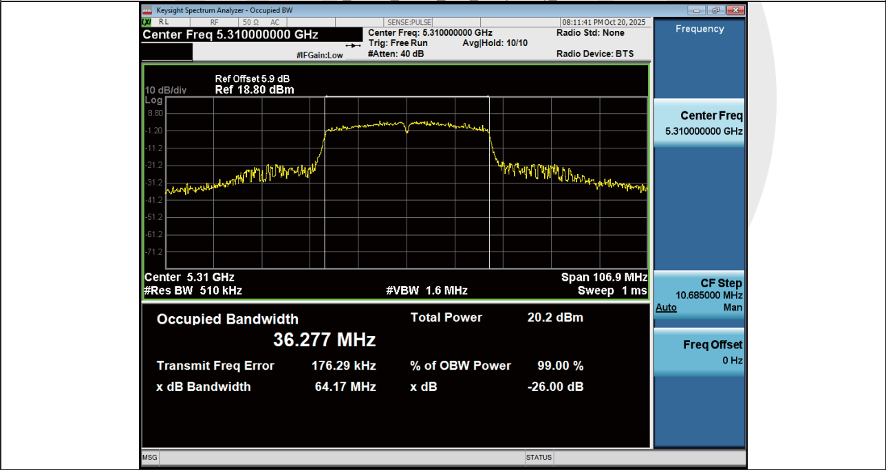
-26BW_NVNT_ANT1_802_11n(HT40)_5310
