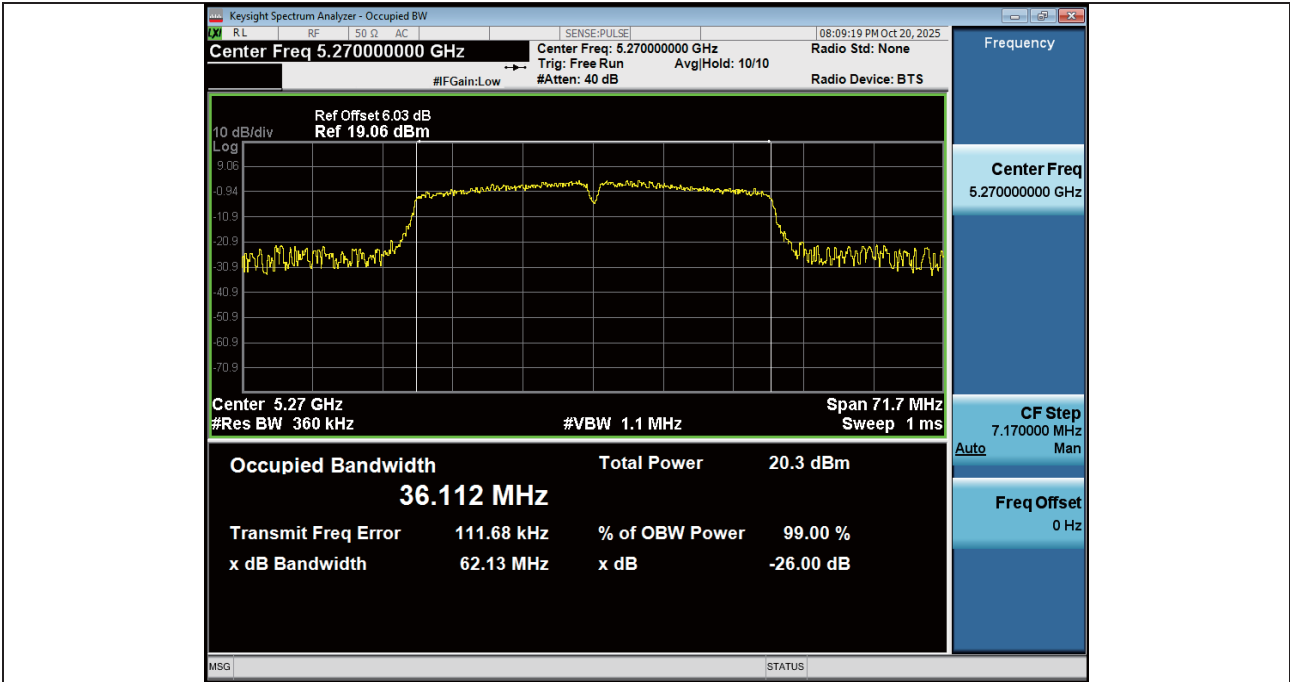
-26BW_NVNT_ANT1_802_11n(HT40)_5270
