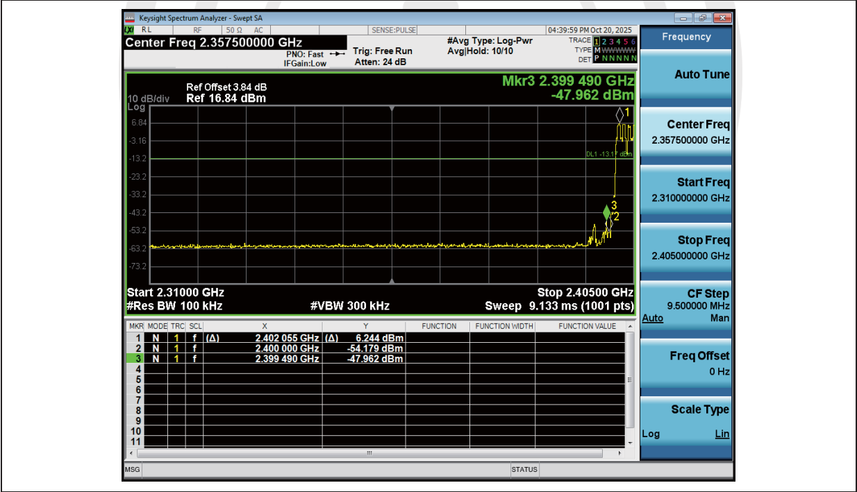
2_Band_Edge_(Hopping)_NVNT_ANT1_2-DH1_Hopping
