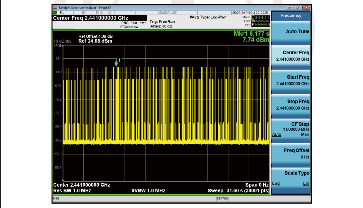
Dwell_Time_(Hopping)_NVNT_ANT1_1-DH5_2441_00_Accumulated
