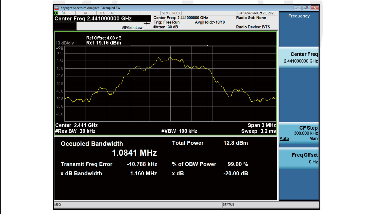
-20dB_Bandwidth_NVNT_ANT1_3-DH1_2441_00
