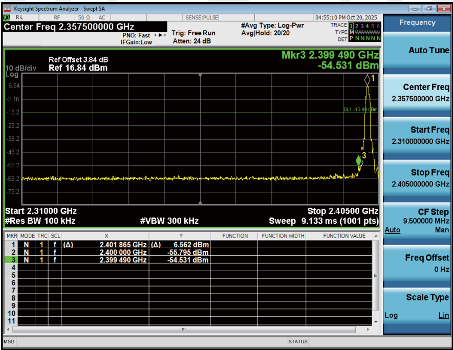
2_Bandedge_NVNT_ANT1_3-DH1_2402_00
