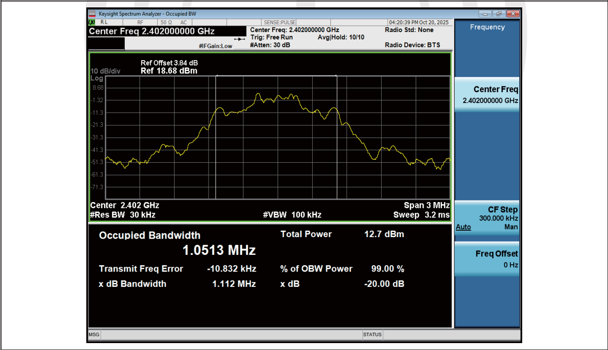
-20dB_Bandwidth_NVNT_ANT1_2-DH1_2402_00
