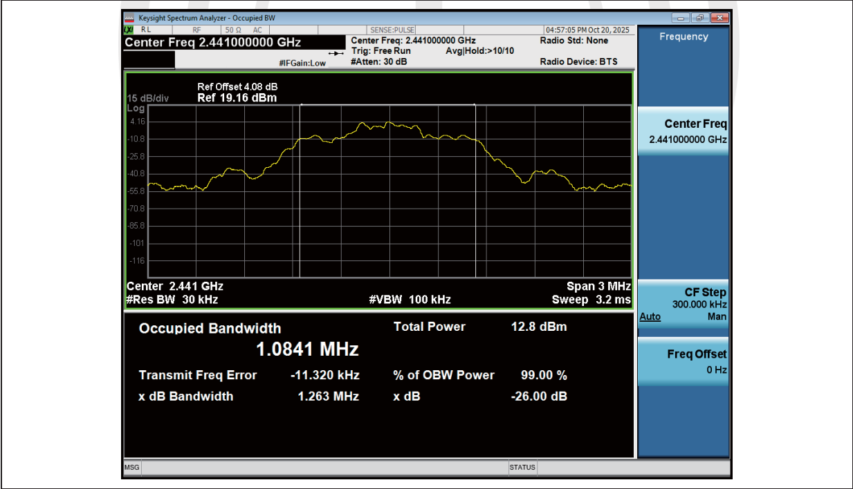
99%_Occupied_Bandwidth_NVNT_ANT1_3-DH1_2441_00
