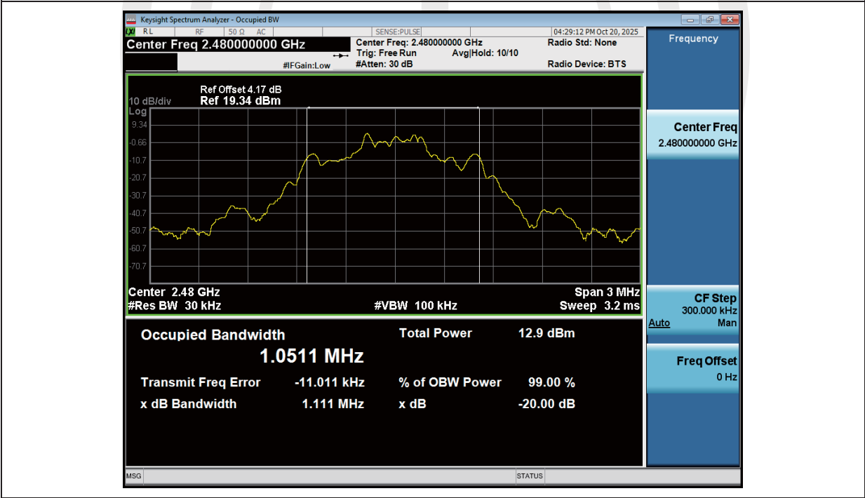
-20dB_Bandwidth_NVNT_ANT1_2-DH1_2480_00
