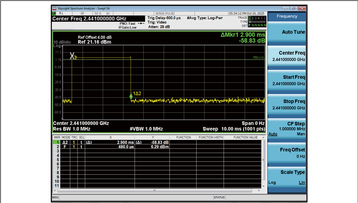
Dwell_Time_(Hopping)_NVNT_ANT1_3-DH5_2441_00_Accumulated
