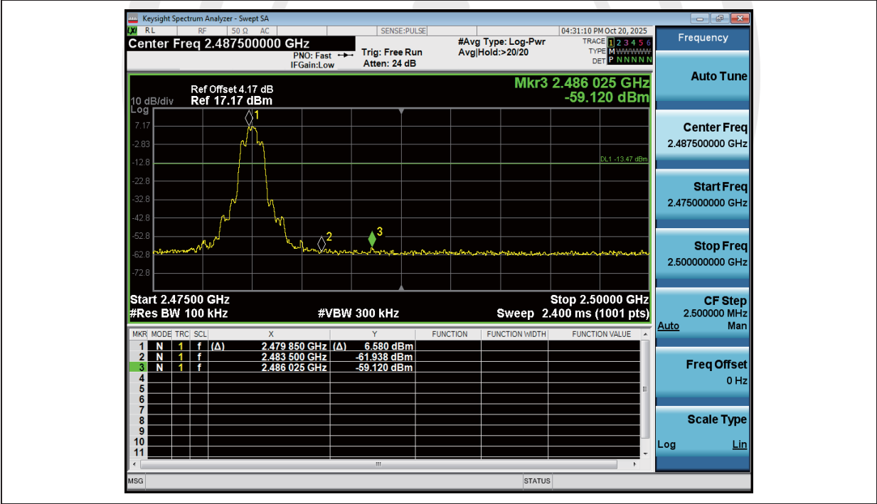
2_Bandedge_NVNT_ANT1_2-DH1_2480_00
