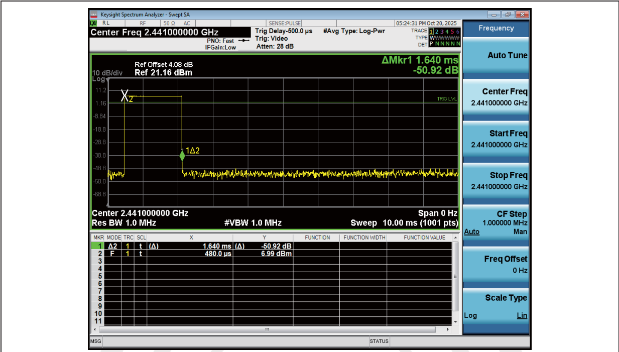
Dwell_Time_(Hopping)_NVNT_ANT1_1-DH3_2441_00_Accumulated
