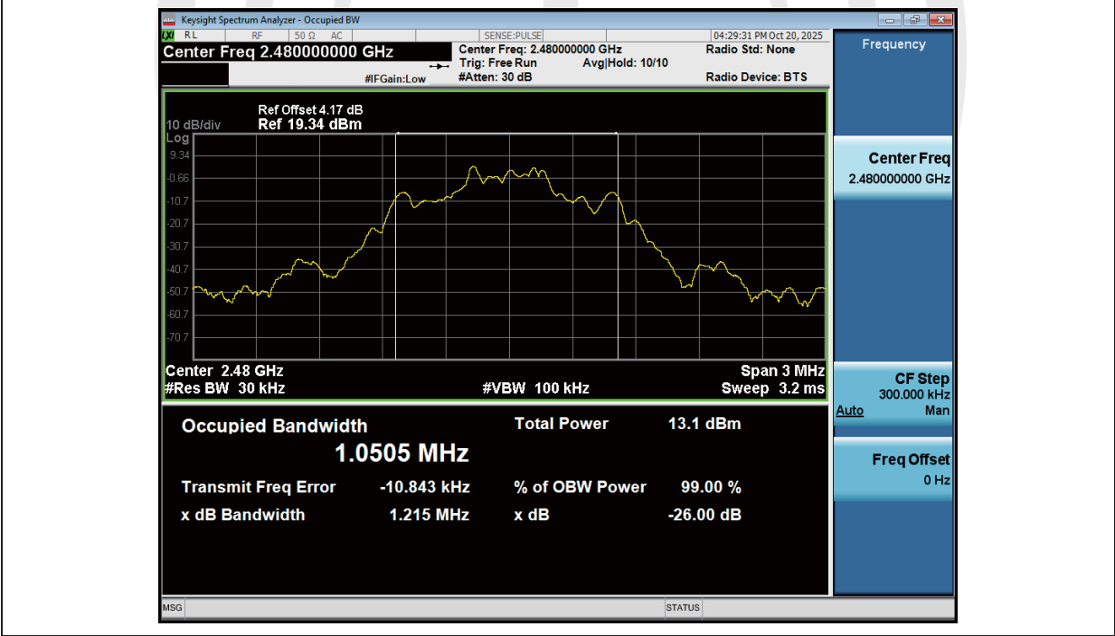
99%_Occupied_Bandwidth_NVNT_ANT1_2-DH1_2480_00
