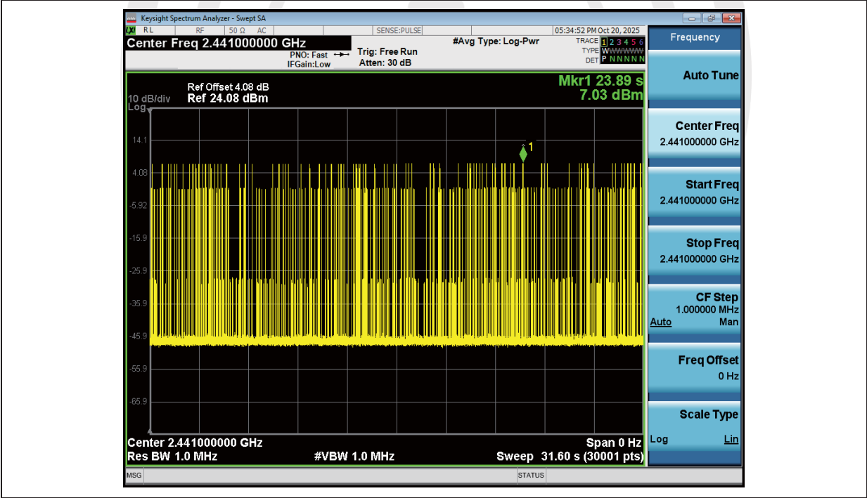
Dwell_Time_(Hopping)_NVNT_ANT1_3-DH5_2441_00_Accumulated
