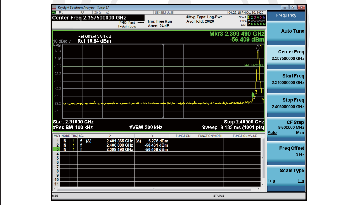
2_Bandedge_NVNT_ANT1_2-DH1_2402_00
