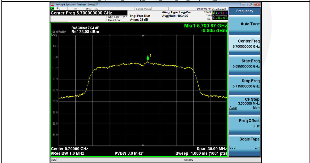
Power Spectral Density NVNT_ANT1_802_11n(HT20)_5700
