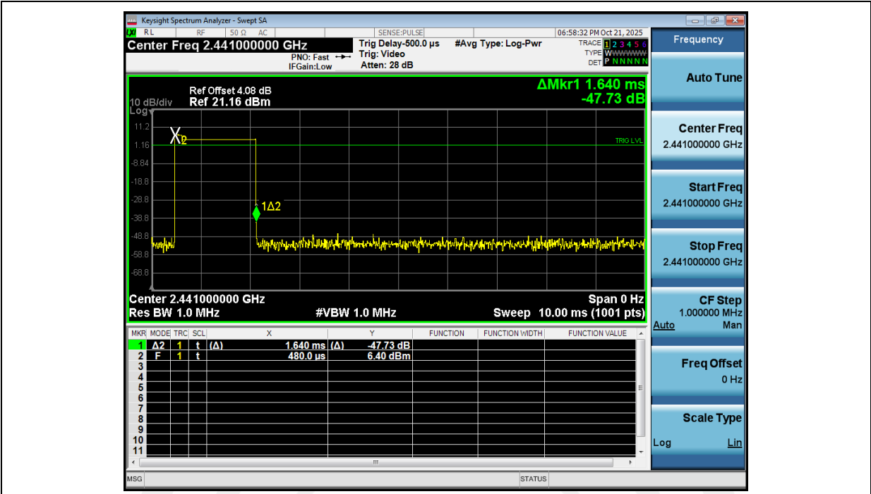
Dwell_Time_(Hopping)_NVNT_ANT1_2-DH3_2441_00_Accumulated
