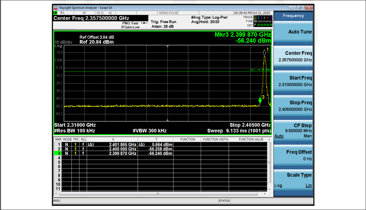
2_Bandedge_NVNT_ANT1_3-DH1_2402_00
