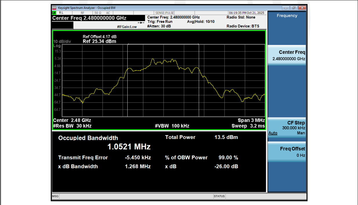
99%_Occupied_Bandwidth_NVNT_ANT1_2-DH1_2480_00
