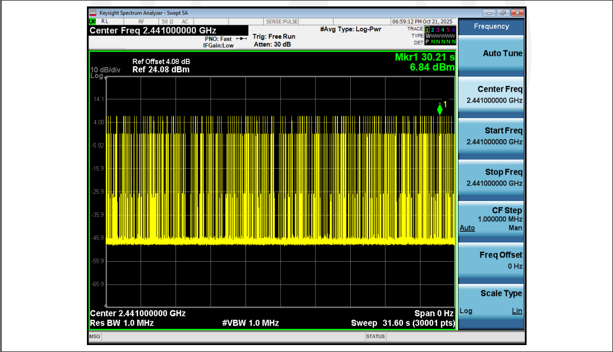
Dwell_Time_(Hopping)_NVNT_ANT1_2-DH3_2441_00_Accumulated
