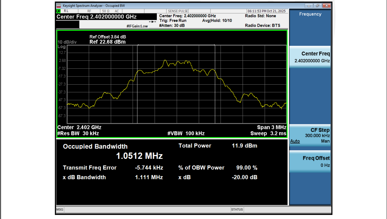
-20dB_Bandwidth_NVNT_ANT1_2-DH1_2402_00
