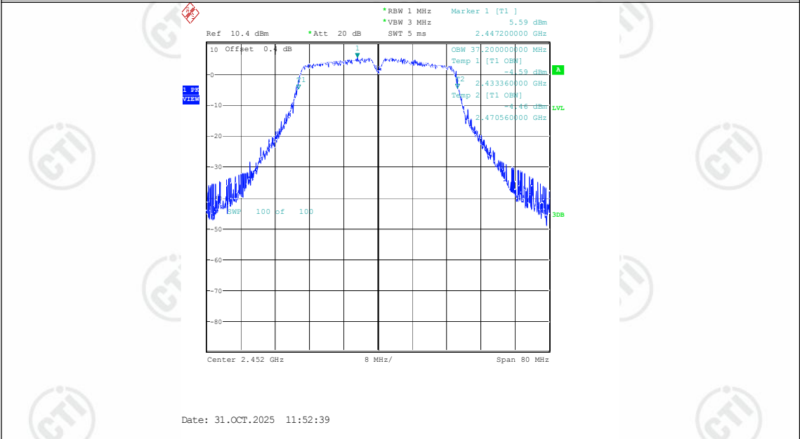
11N40SISO-Ant1-2452
