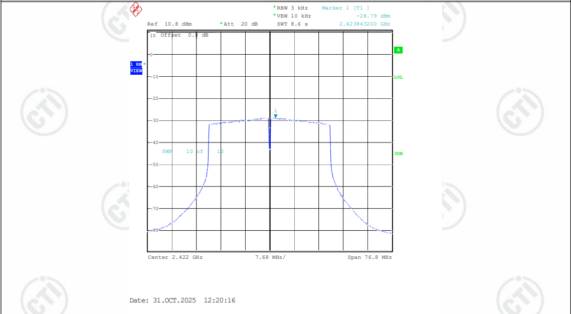
11AX40SISO-Ant1-2422-PASS
