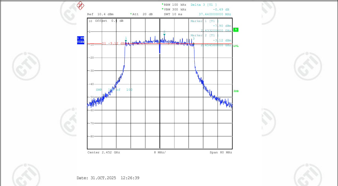
11AX40ISO-Ant1-2452-PASS
