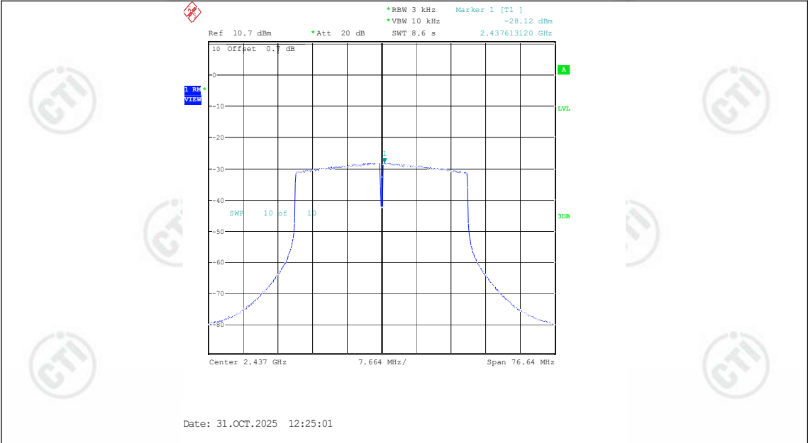
11AX40SISO-Ant1-2437-PASS
