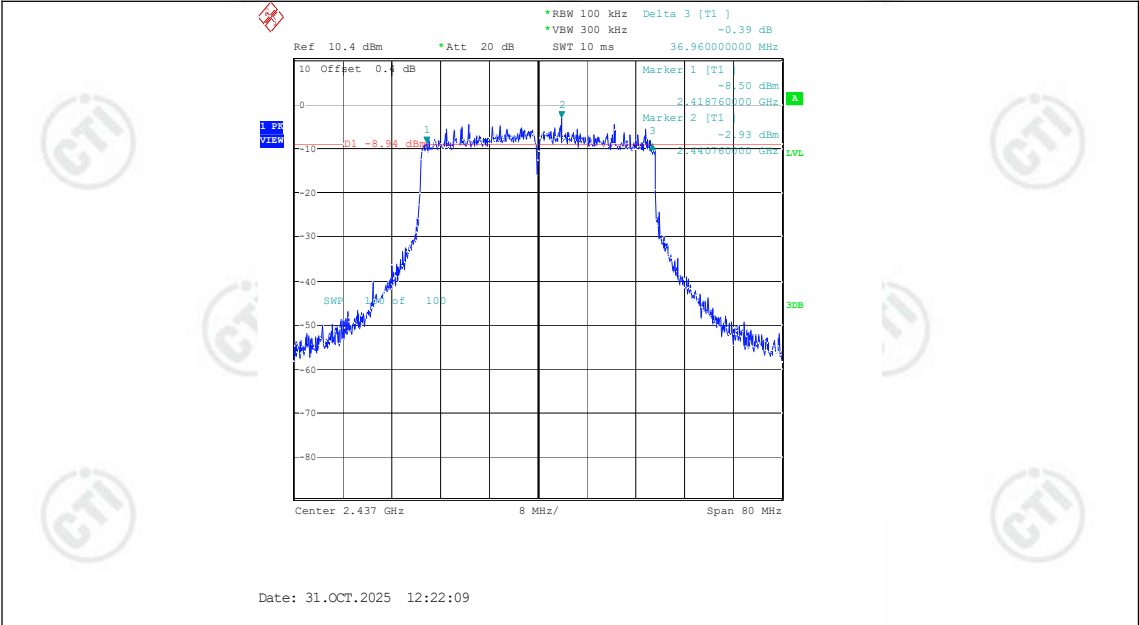
11AX40ISO-Ant1-2437-PASS
