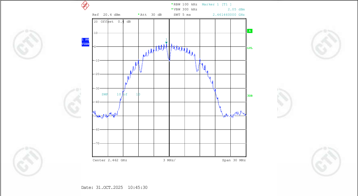
11B-Ant1-2462-0~Reference-PASS
