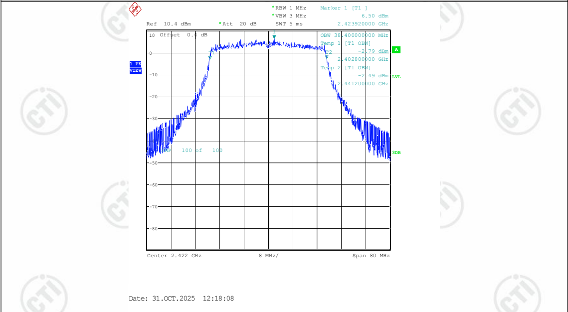
11AX40SISO-Ant1-2422
