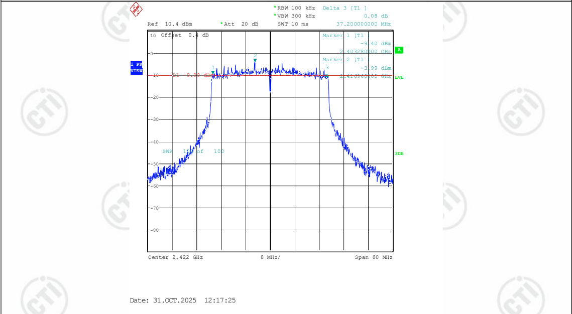
11AX40ISO-Ant1-2422-PASS
