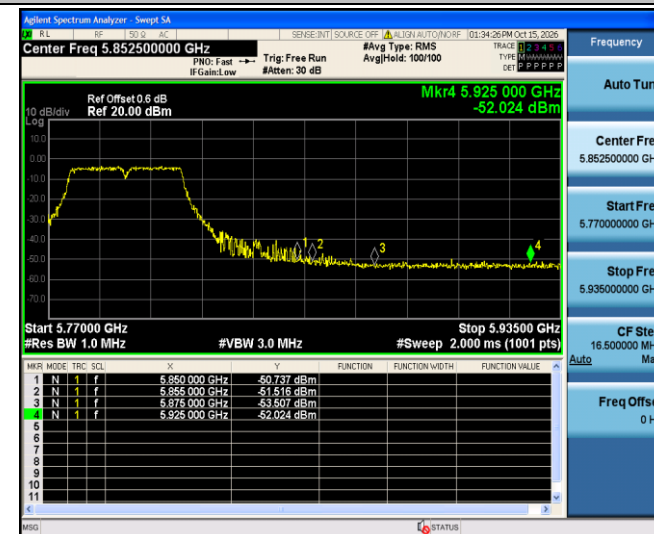
11AC40SISO_Ant1_High_5795_Peak
