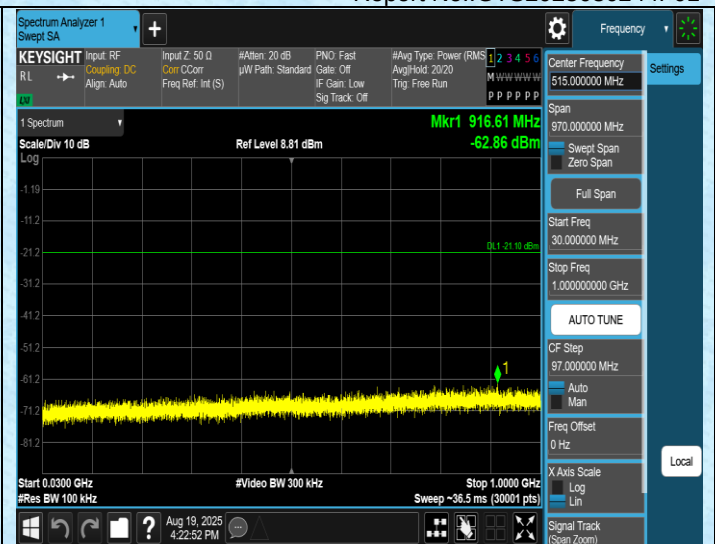
11N20SISO-Ant1-2462-30~1000-PASS
