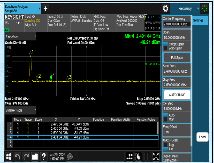
DH5-Ant1-2480-PASS
