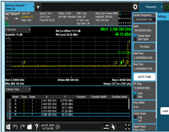
DH5-Ant1-2402-PASS
