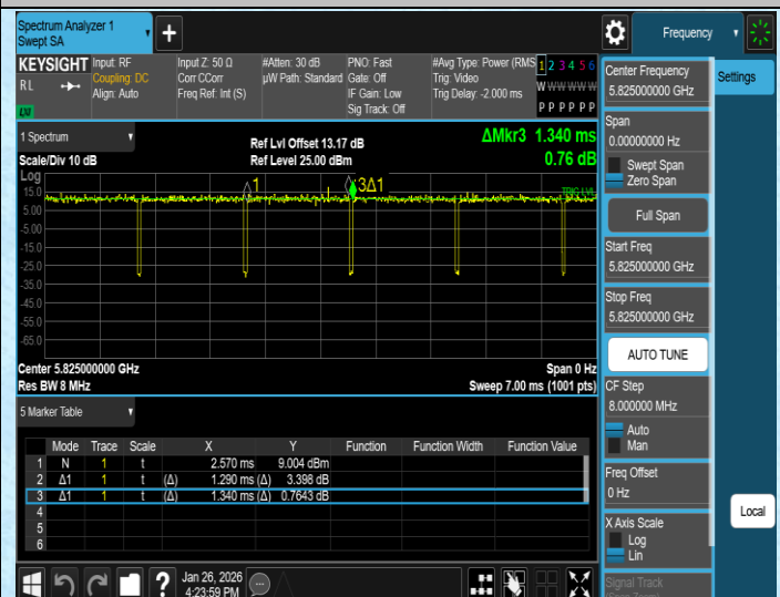
NTNV-11N20SISO-Ant1-5825
