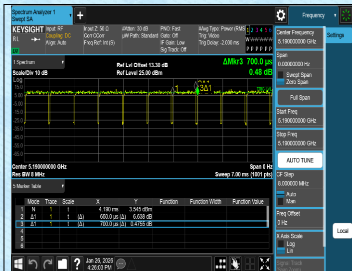
NTNV-11N40SISO-Ant1-5190
