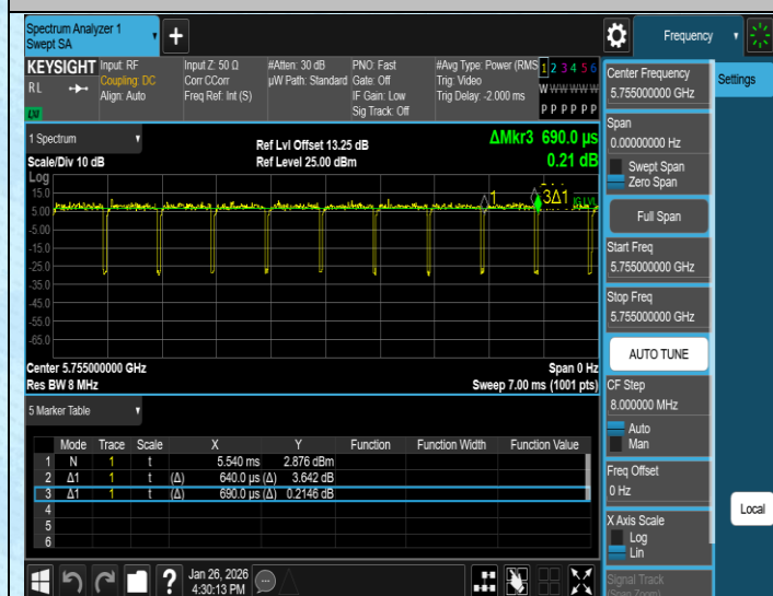
NTNV-11N40SISO-Ant1-5755
