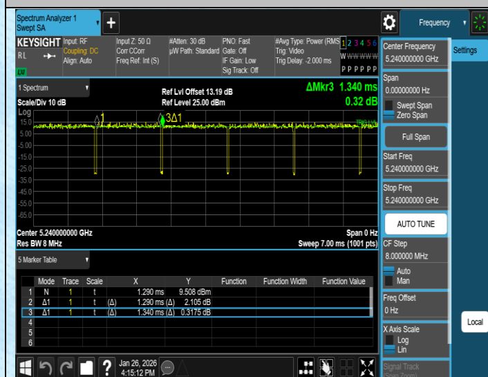
NTNV-11N20SISO-Ant1-5240
