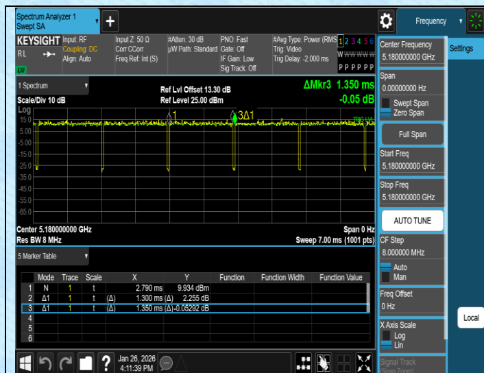
NTNV-11N20SISO-Ant1-5180
