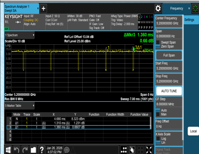
NTNV-11AC20SISO-Ant1-5200
