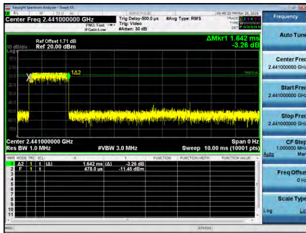
Burst(3DH3)
