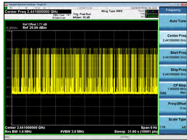
Accumulate(3DH3)
