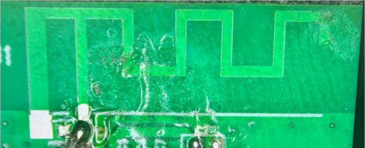
Physical appearance and physical dimensions of the antenna
