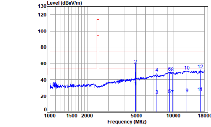
2.4G_SRD_HIGH_TX_Horizontal
