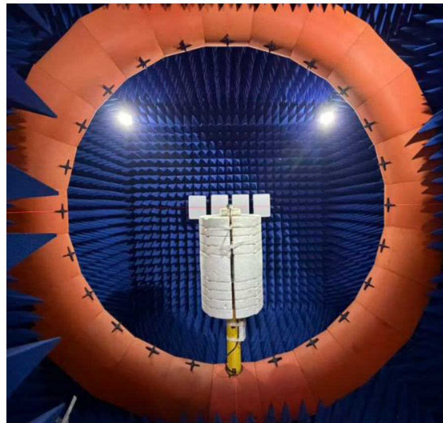
Testing 3D microwave darkroom(3m*3m*3m)
