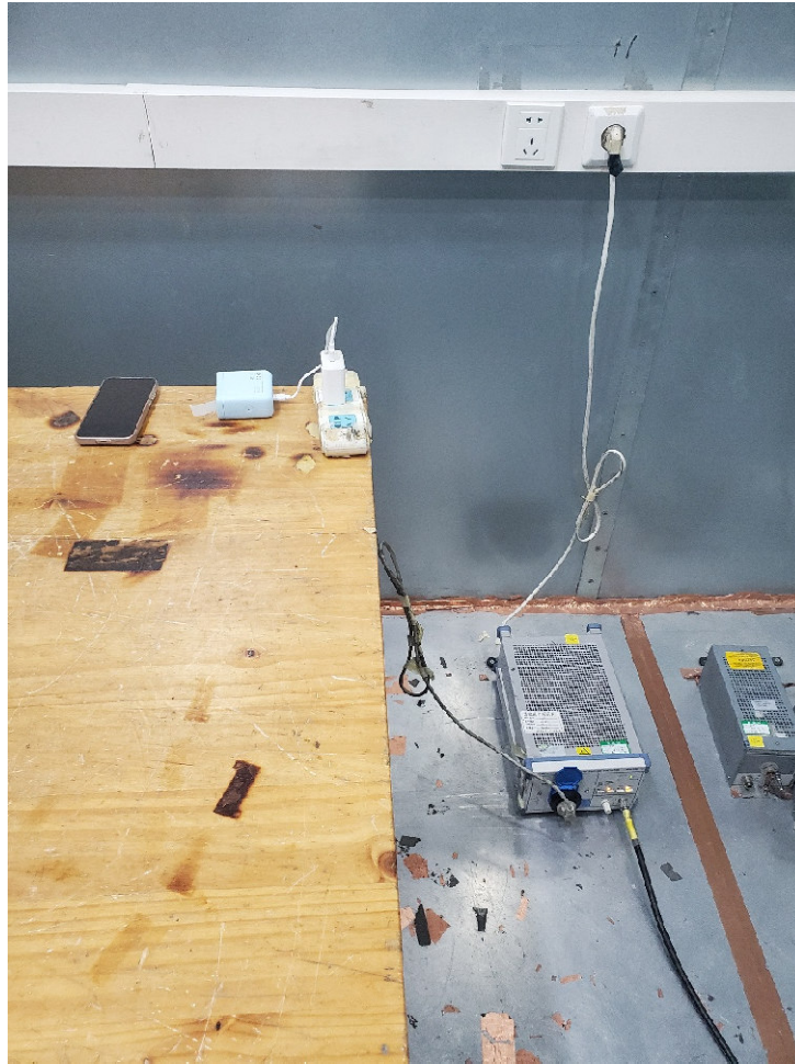
Picture 2: Conducted Emissions Test Setup
