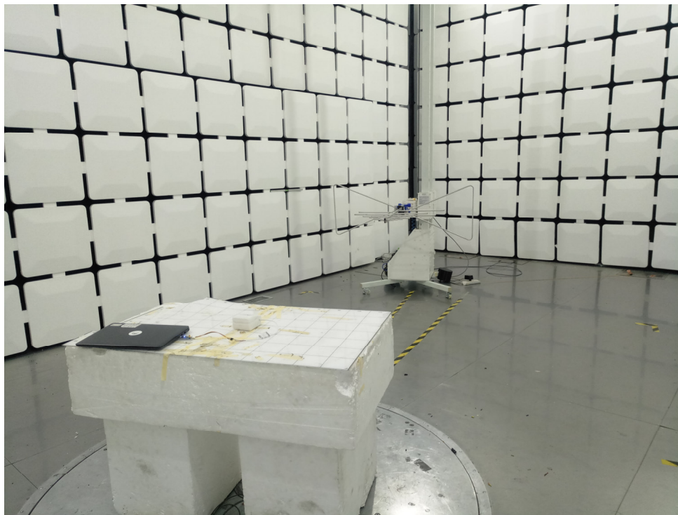
30MHz-1GHz
