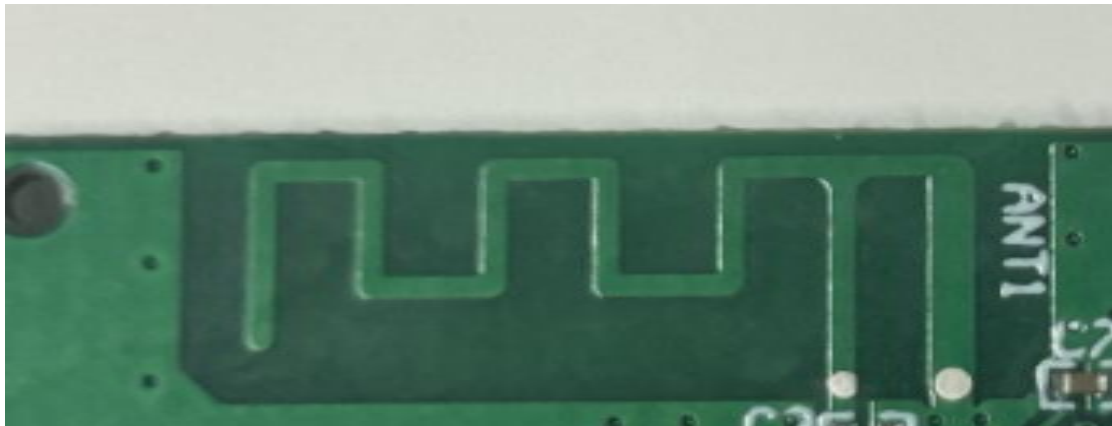
Antenna physical unit and dimensions (Unit: mm)
