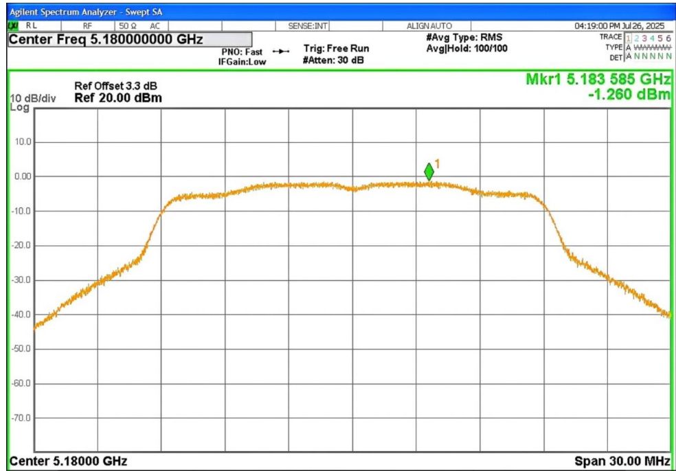
PSD NVNT ac20 5180MHz Ant1
