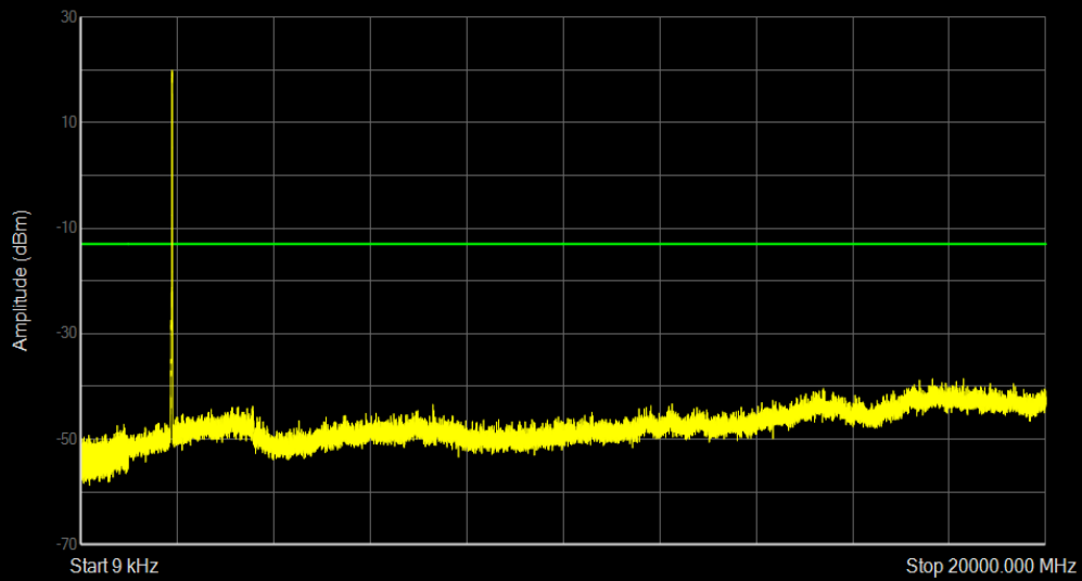
Band25 QPSK BW=10MHz Channel=26640 RB Size=50 Position=#0
