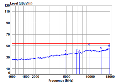
BLE_1M_TX_CH_19_Horizontal-Avg
