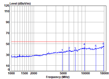
BLE_1M_TX_CH_19_Vertical-Avg
