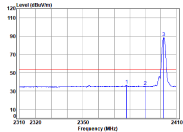
BLE_1M_TX_CH_00_Horizontal-Avg
