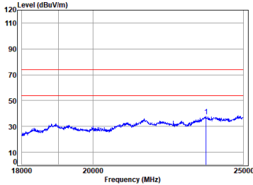
BLE_1M_TX_CH_19_Vertical-Peak
