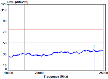
BLE_1M_TX_CH_19_Horizontal-Peak
