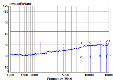
BT_DH5_TX_CH_39_Vertical
