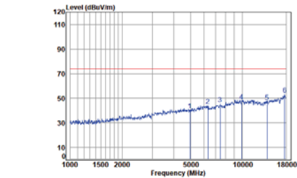
Right BLE_2M_TX_CH_38_Vertical-Peak
