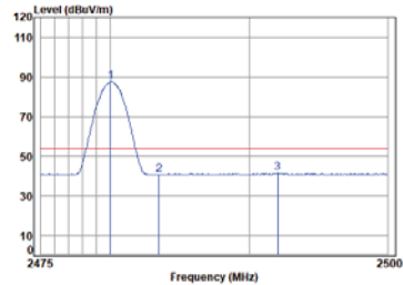
Right BLE_1M_TX_CH_39_Vertical-Avg
