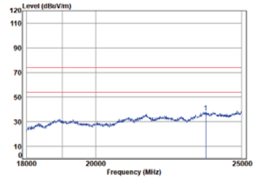
Right BLE_1M_TX_CH_19_Vertical-Peak
