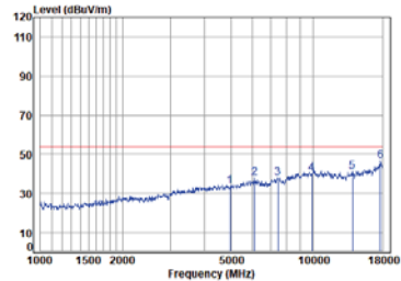
Right BLE_1M_TX_CH_39_Horizontal-Avg
