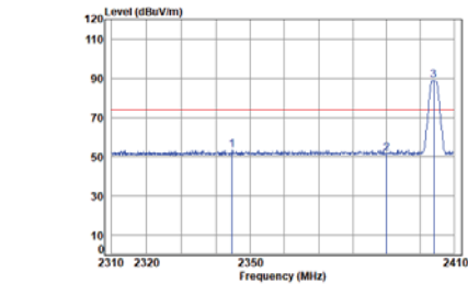
Right BLE_2M_TX_CH_01_Vertical-Peak
