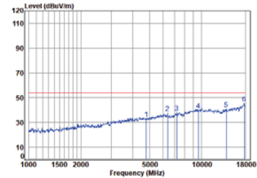
Right BLE_1M_TX_CH_00_Vertical-Avg
