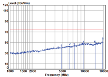
Left BLE_1M_TX_CH_19_Vertical-Peak
