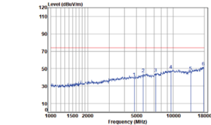
Right BLE_2M_TX_CH_01_Horizontal-Peak
