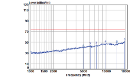
Right BLE_2M_TX_CH_38_Horizontal-Peak
