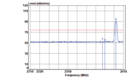
Left BLE_1M_TX_CH_00_Vertical-Peak
