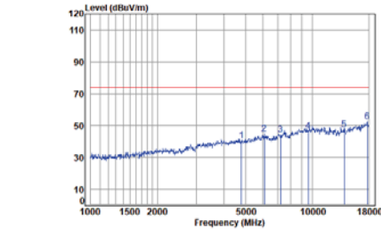
Right BLE_1M_TX_CH_00_Vertical-Peak
