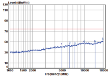
Right BLE_1M_TX_CH_39_Horizontal-Peak
