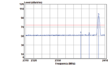
Left BLE_1M_TX_CH_00_Horizontal-Peak
