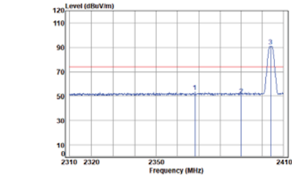
Right BLE_2M_TX_CH_01_Horizontal-Peak
