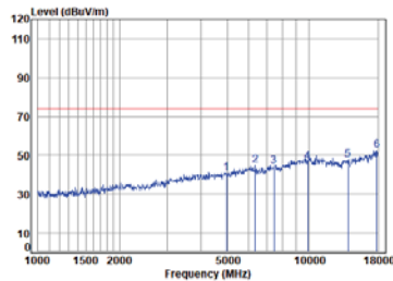
Left BLE_2M_TX_CH_38_Horizontal-Peak
