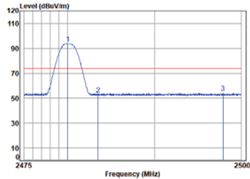
Left BLE_1M_TX_CH_39_Vertical-Peak
