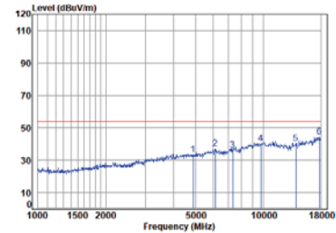
Right BLE_2M_TX_CH_19_Vertical-Avg
