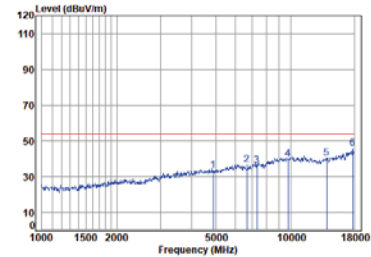
Right BLE_1M_TX_CH_19_Vertical-Avg
