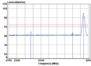
Left BLE_2M_TX_CH_01_Horizontal-Peak
