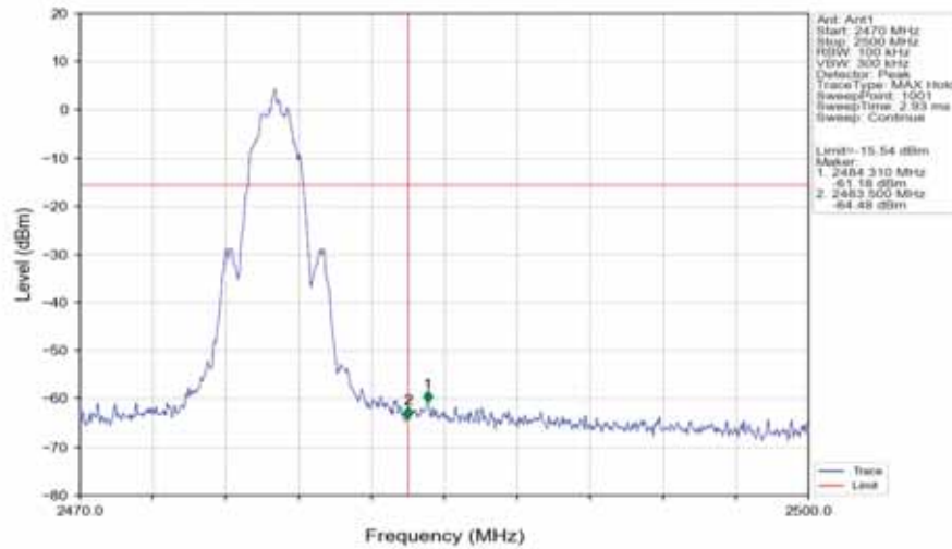
2M_HCH_2478MHz_Ant1_NTNV
