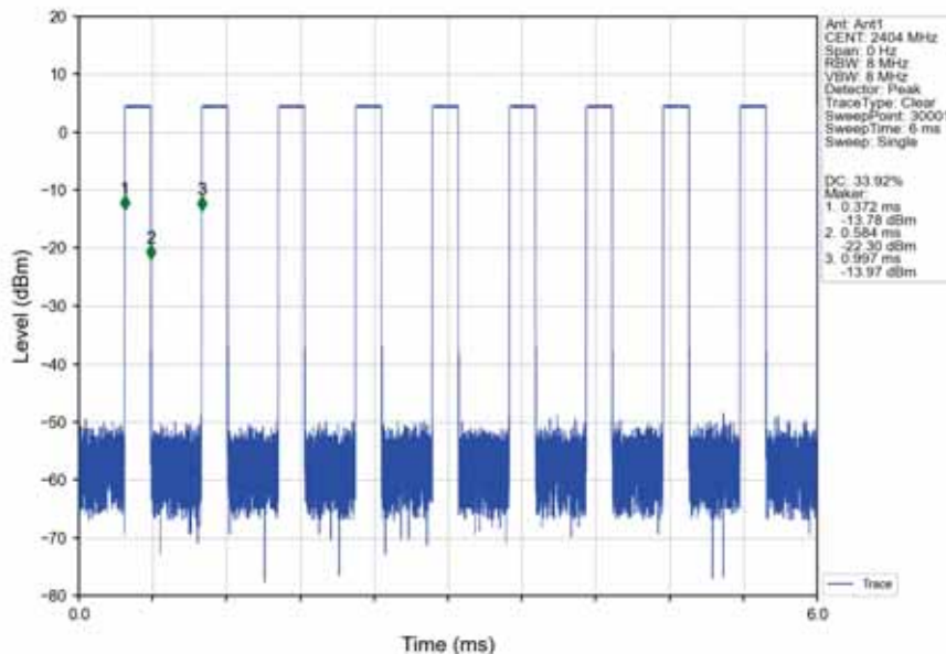
2M_LCH_2404MHz_Ant1_NTNV
