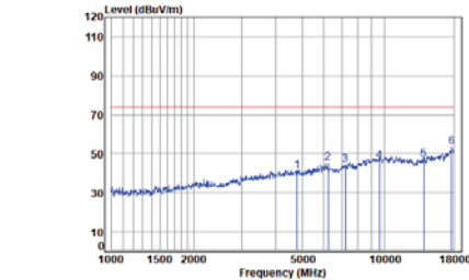
Right BLE_1M_TX_CH_00_Horizontal-Peak
