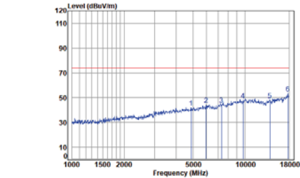
Right BLE_1M_TX_CH_19_Vertical-Peak
