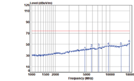
Left BLE_1M_TX_CH_00_Horizontal-Peak
