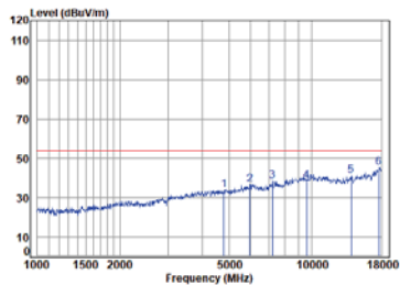
Left BLE_1M_TX_CH_00_Vertical-Avg
