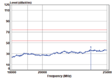
Left BLE_1M_TX_CH_19_Vertical-Peak
