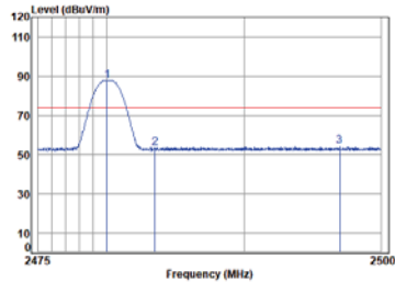
Right BLE_1M_TX_CH_39_Vertical-Peak
