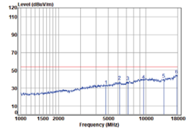
Right BLE_1M_TX_CH_00_Horizontal-Avg
