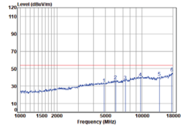
Right BLE_1M_TX_CH_19_Horizontal-Avg
