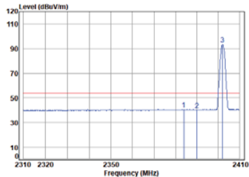
Left BLE_1M_TX_CH_00_Horizontal-Avg
