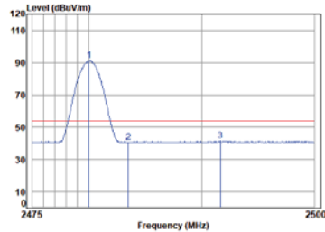
Left BLE_1M_TX_CH_39_Vertical-Avg
