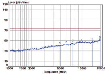
Right BLE_1M_TX_CH_39_Vertical-Peak
