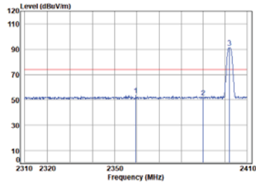
Right BLE_1M_TX_CH_00_Horizontal-Peak
