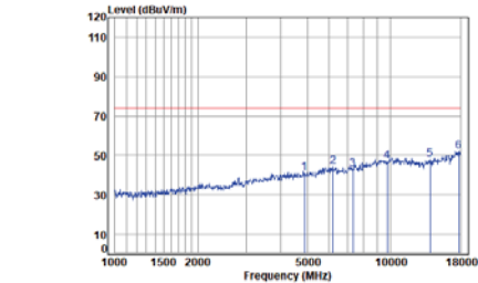
Right BLE_1M_TX_CH_19_Horizontal-Peak
