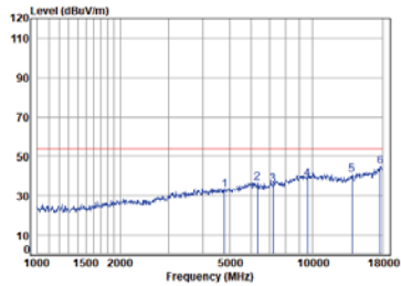
Left BLE_1M_TX_CH_00_Horizontal-Avg
