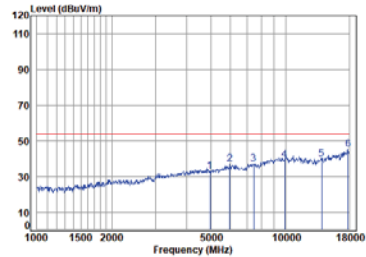
Right BLE_1M_TX_CH_39_Vertical-Avg
