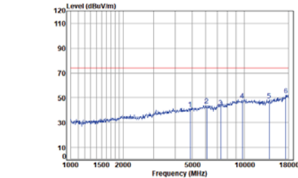
Right BLE_2M_TX_CH_19_Horizontal-Peak
