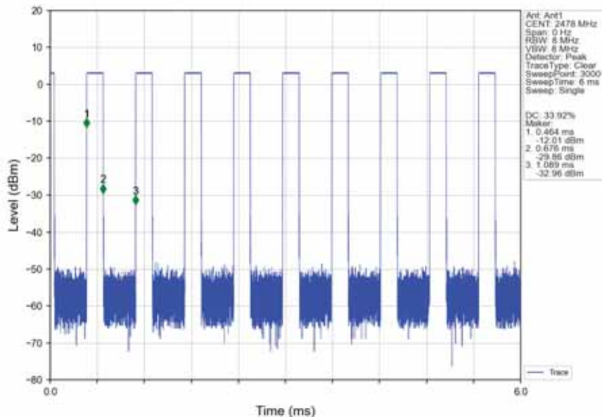
2M_HCH_2478MHz_Ant1_NTNV
