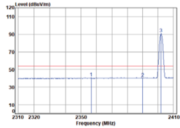
Right BLE_1M_TX_CH_00_Horizontal-Avg
