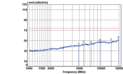
Right BLE_2M_TX_CH_19_Vertical-Peak
