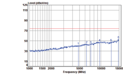
Right BLE_2M_TX_CH_01_Vertical-Peak
