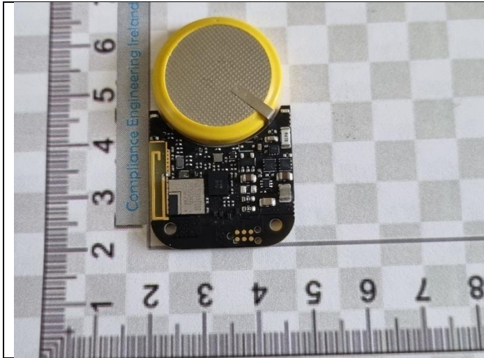
Fig A1: Node Host pcb top side
