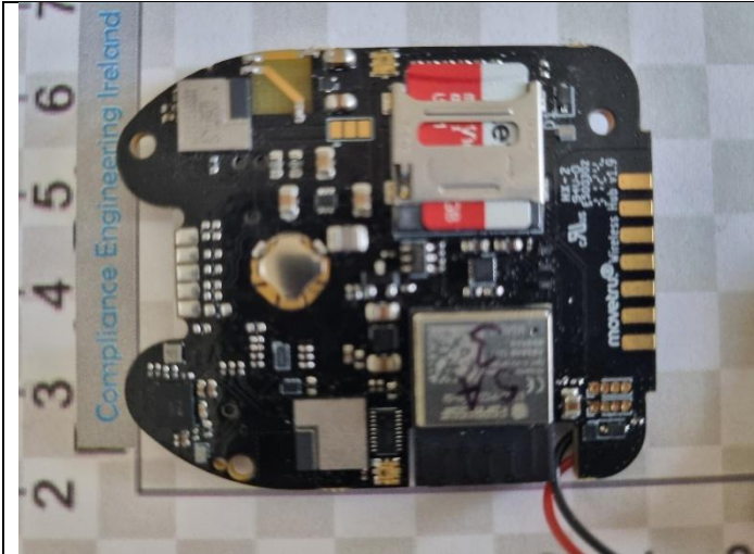
Fig A4: Hub host pcb top side
