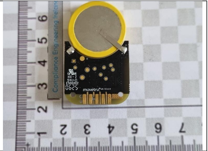
Fig A2: Node host pcb bottom side
