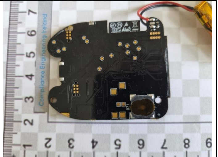
Fig A5: Hub Host pcb bottom side
