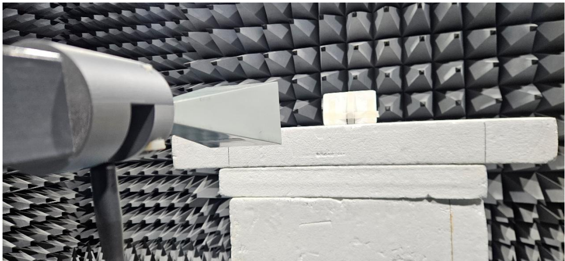
Rad Emission 18GHz -26GHz
