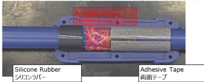
Photo from bottom (After attaching of the strain gauge and connecting to base terminal)
