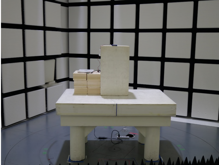
Photograph 7: Set-up for Radiated Spurious Emission above 1GHz, Front View
