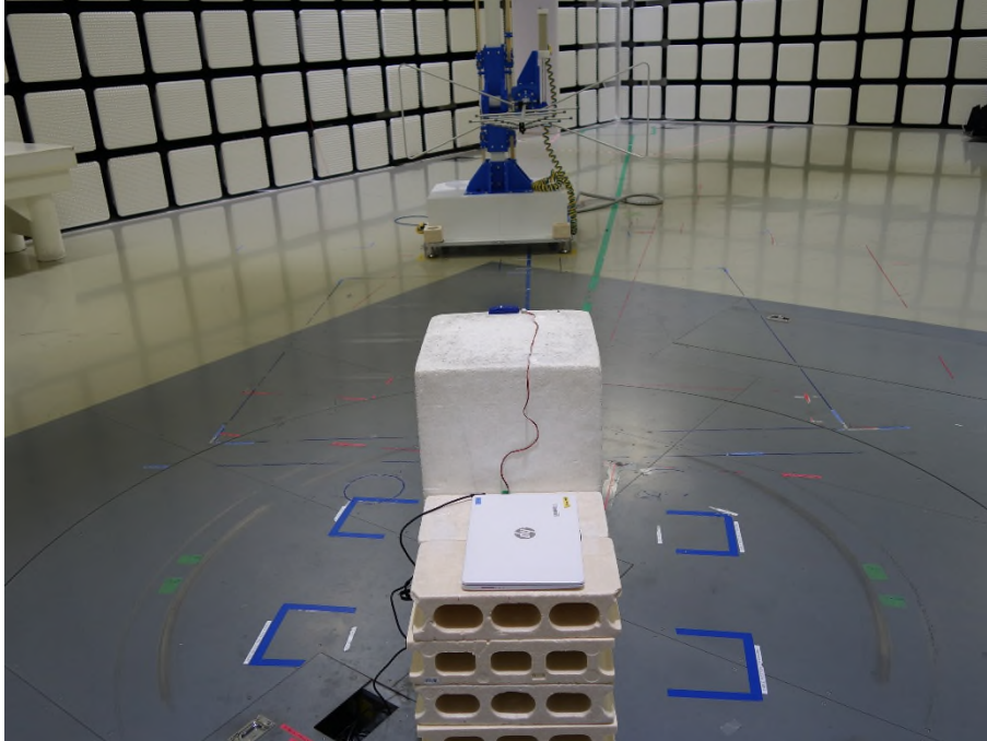
Photograph 5: Set-up for Radiated Spurious Emission below 1GHz, Front View
