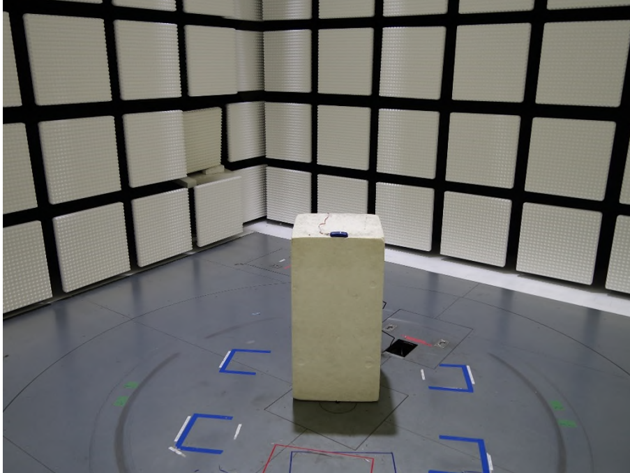
Photograph 3: Set-up for Radiated Spurious Emission below 30MHz, Front View
