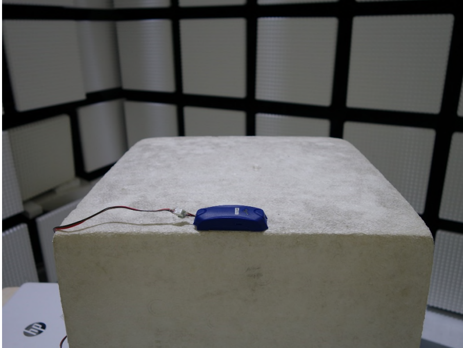
Photograph 11: Set-up for Z-Axis of the EUT
