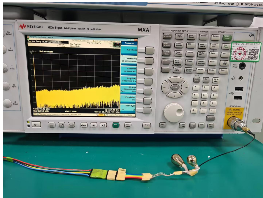
RF Conducted
