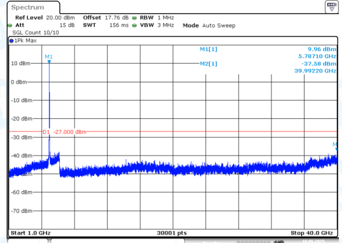
11AC40MIMO-Ant2-5795-1000~40000-PASS
