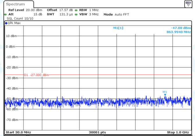
11AC20MIMO-Ant2-5240-30~1000-PASS
