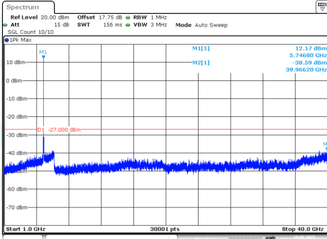
11AC20MIMO-Ant1-5745-1000~40000-PASS
