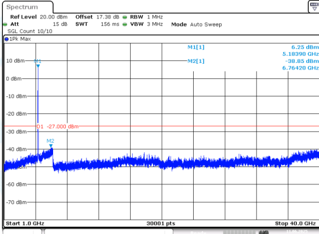
11AC40MIMO-Ant1-5190-1000~40000-PASS
