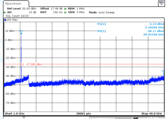
11AC40MIMO-Ant2-5190-1000~40000-PASS
