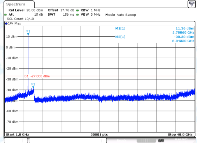
11N20MIMO-Ant2-5785-1000~40000-PASS
