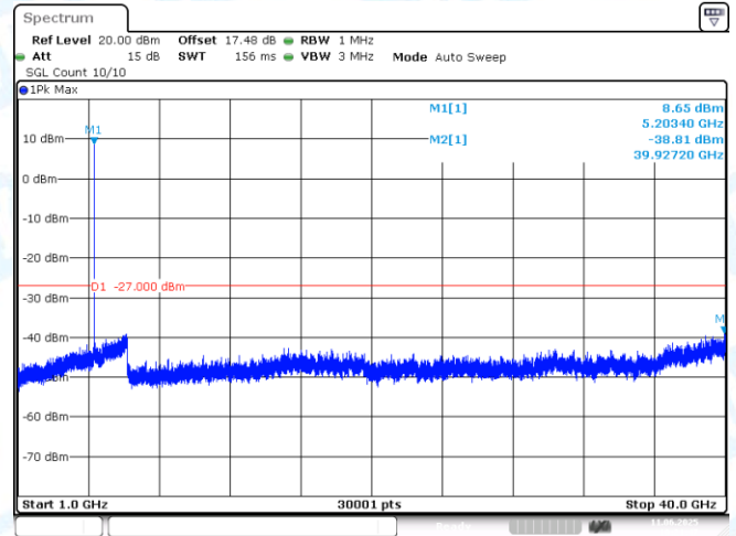
11N20MIMO-Ant2-5200-1000~40000-PASS
