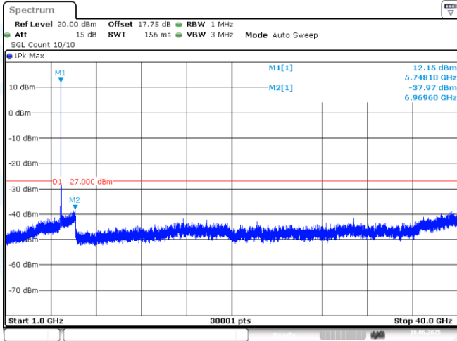
11AX20MIMO-Ant1-5745-1000~40000-PASS
