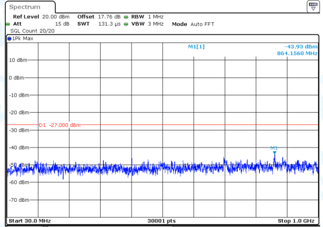
11AC80-CDD-Ant2-5775-30~1000-PASS
