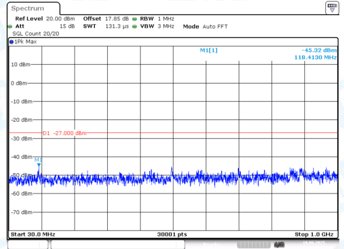
11AX20MIMO-Ant2-5825-30~1000-PASS
