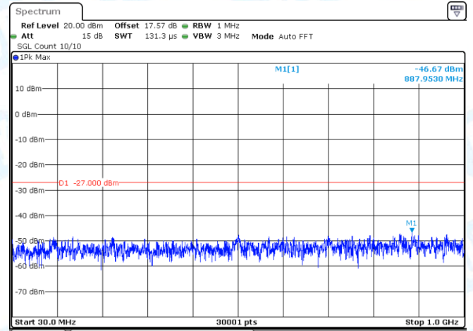
11AX20MIMO-Ant2-5240-30~1000-PASS
