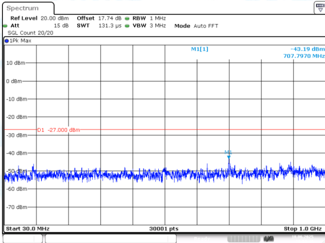
11AX20MIMO-Ant1-5825-30~1000-PASS
