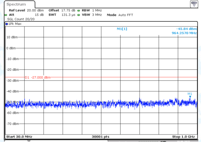
11AX40MIMO-Ant2-5755-30~1000-PASS
