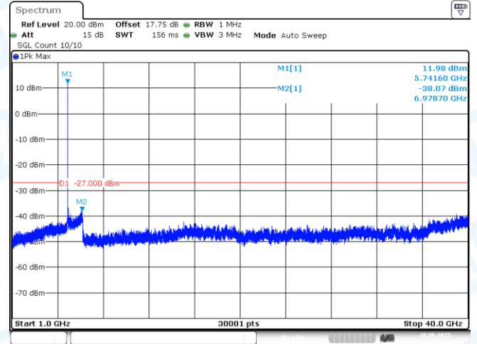
11AX20MIMO-Ant2-5745-1000~40000-PASS
