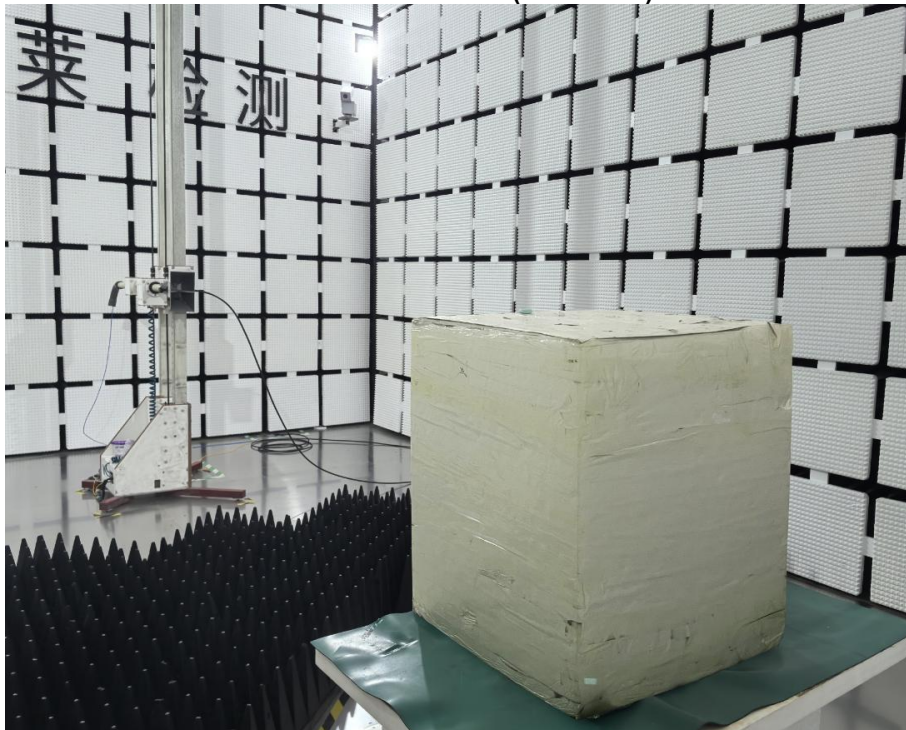
Radiated Emission (Above 1G)
