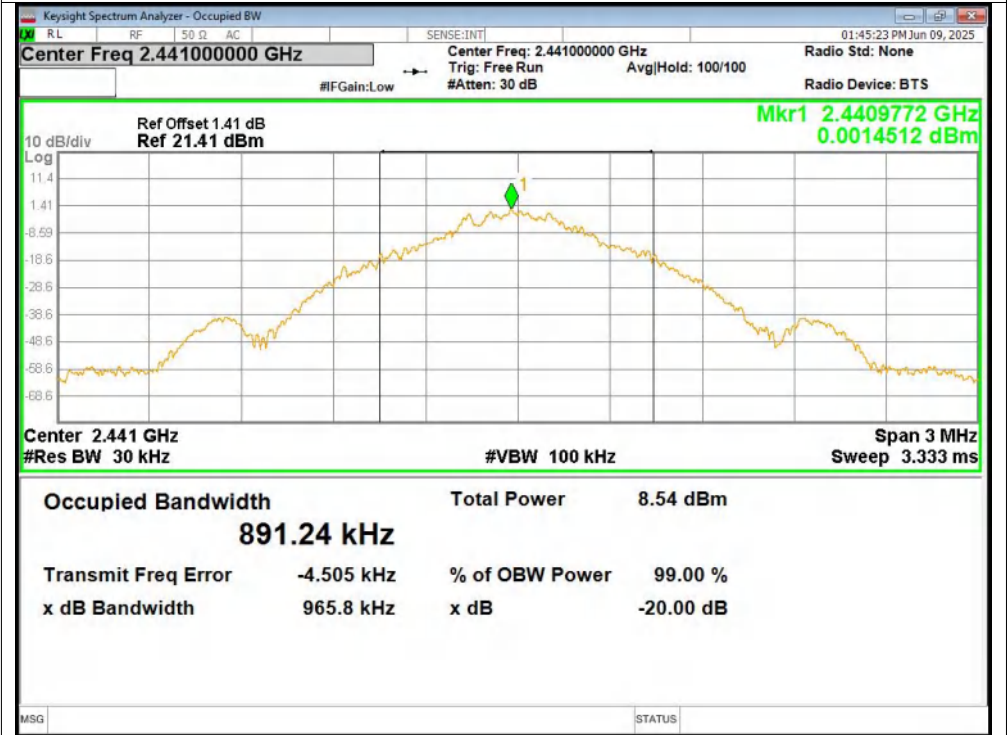
OBW NVNT 1-DH5 2441MHz Ant1
